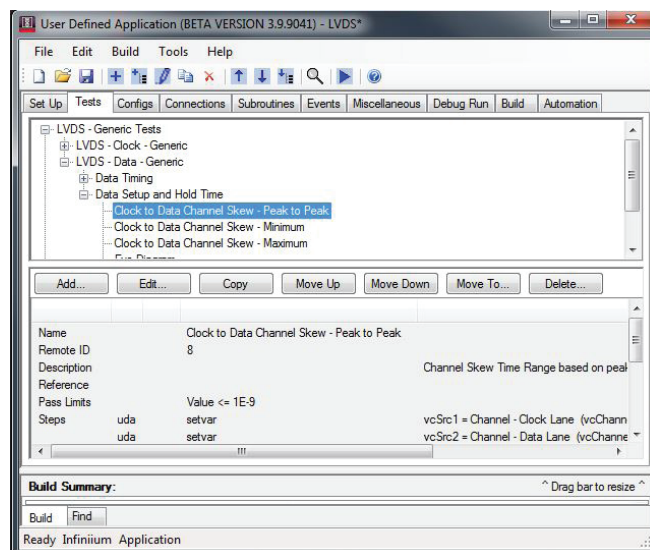
Figure 3. Simple process to create multiple test sequences with individual Pass/Fail results
