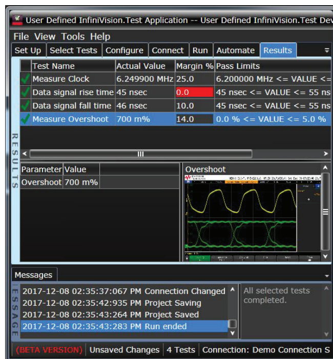
Figure 16. Test results can easily be reviewed, re-run, or executed multiple times before creating a test report
