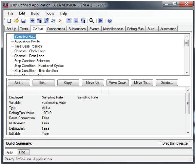
Figure 10. Create, copy, edit your tests and groups of tests
