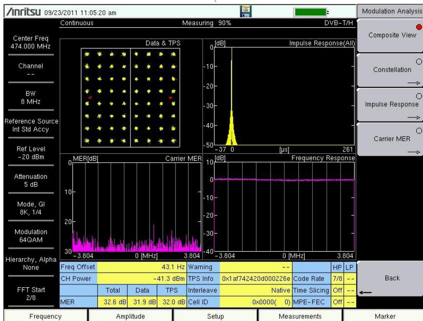
Figure 2-12. Modulation Analysis, Composite View
