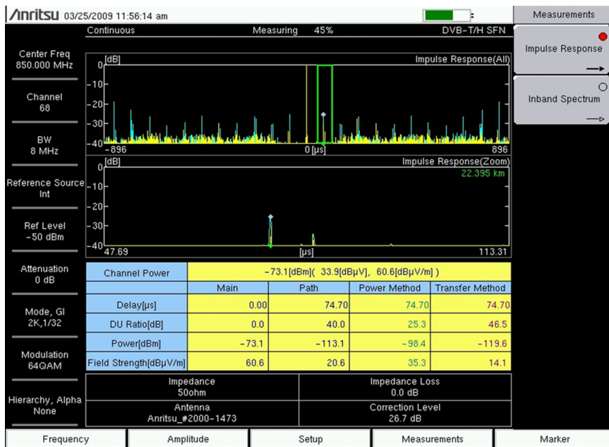
Figure 3-1. Impulse Response Measurement
