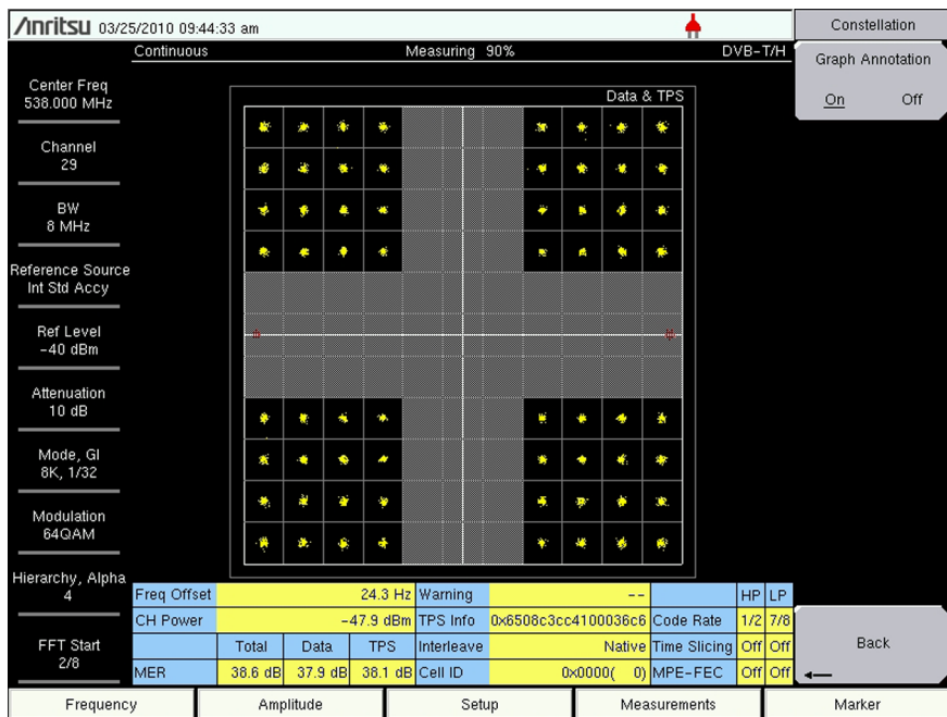
Figure 2-8. 64QAM with Hierarchy set to 4
