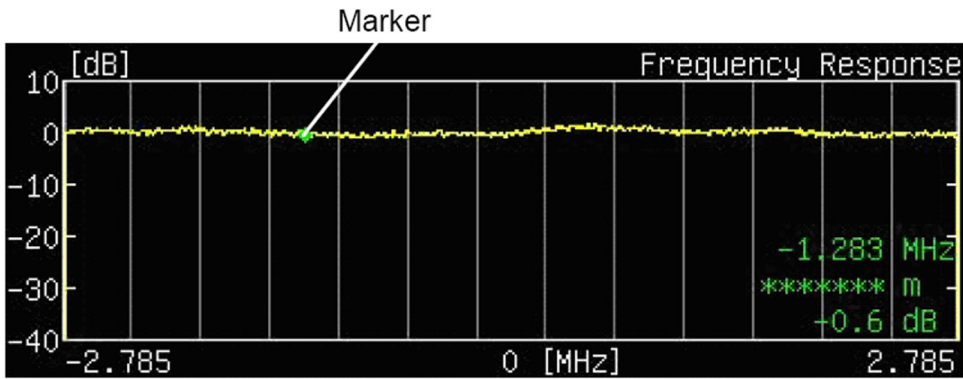
Figure 4-65. Frequency Response Graph with Standard Marker
