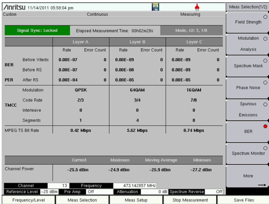
Figure 4-25. BER Measurement Selection
