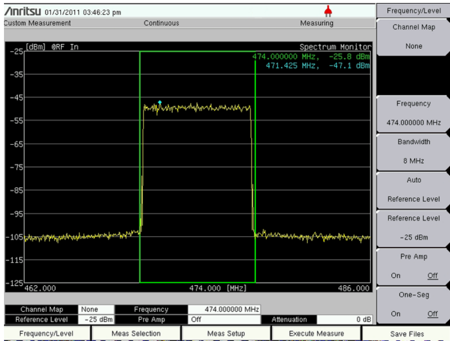
Figure 4-27. Spectrum Monitor with 8 MHz Bandwidth Selected
