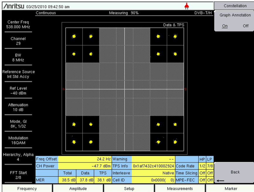
Figure 2-6. 16QAM with Hierarchy set to 4
