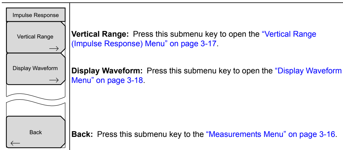
Figure 3-11. Impulse Response Menu
