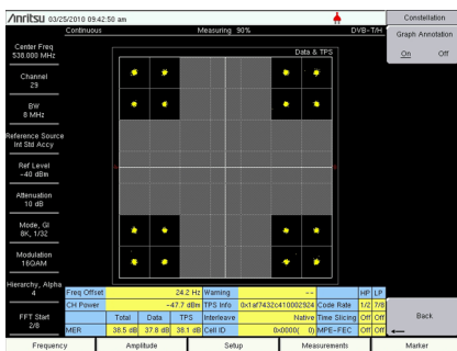
Figure 1-2. DVB-T/H Modulation and Hierarchy Settings
