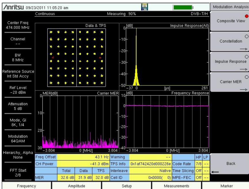
Figure 2-1. A 64QAM Constellation Graph in Composite View
