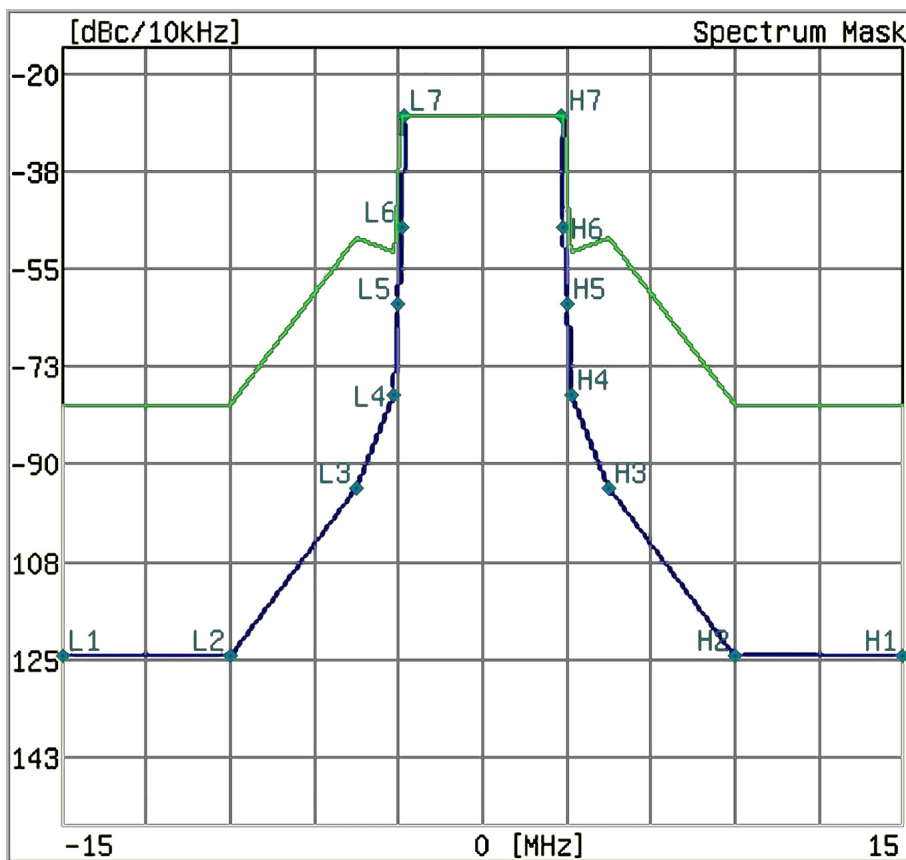
Figure 4-19. Default Filter Data (Green Line) Normalized to -27.4 dB
