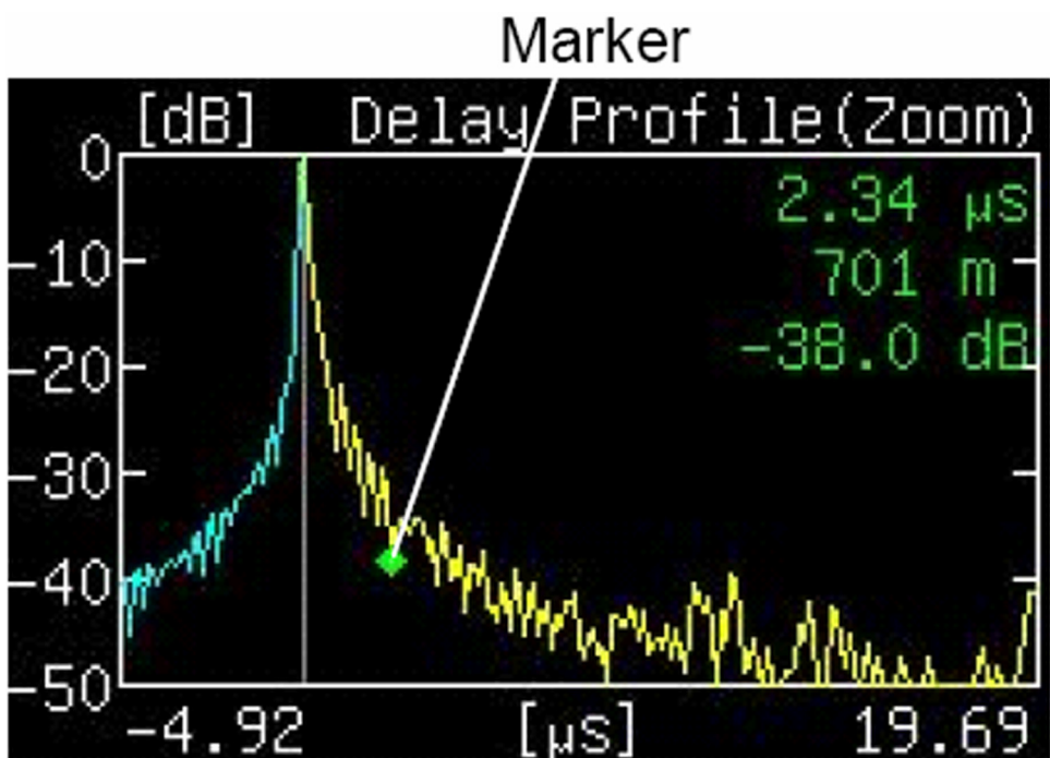
Figure 4-64. Enlarged (Zoom) Graph of Delay Profile
