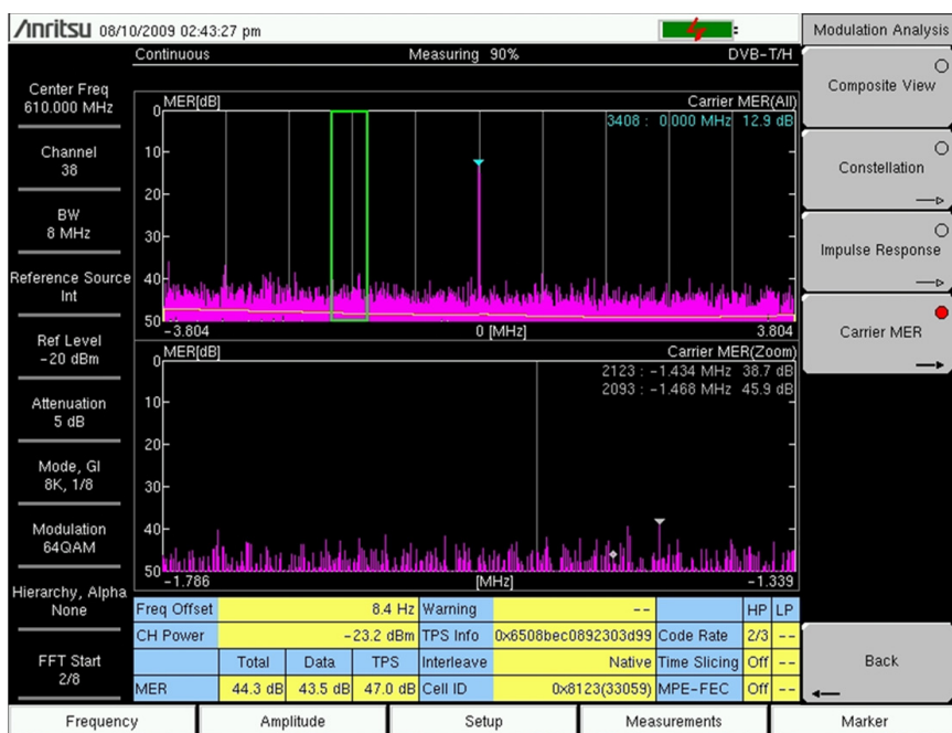
Figure 2-26. Carrier MER
