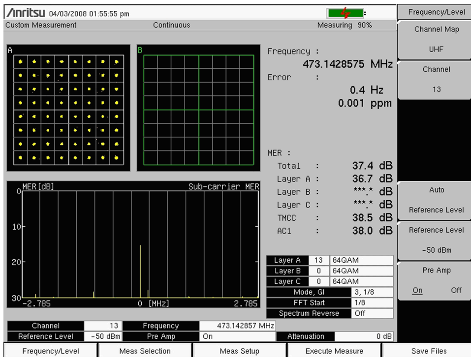
Figure 4-11. Modulation Measurement Screen – Constellation Display
