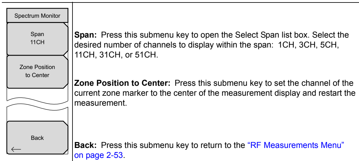
Figure 2-41. Spectrum Monitor Menu
