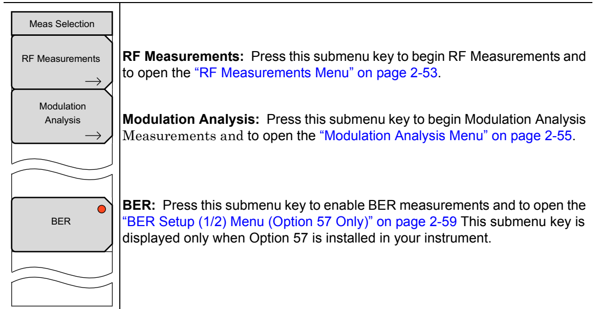
Figure 2-37. Measurement Selection Menu
