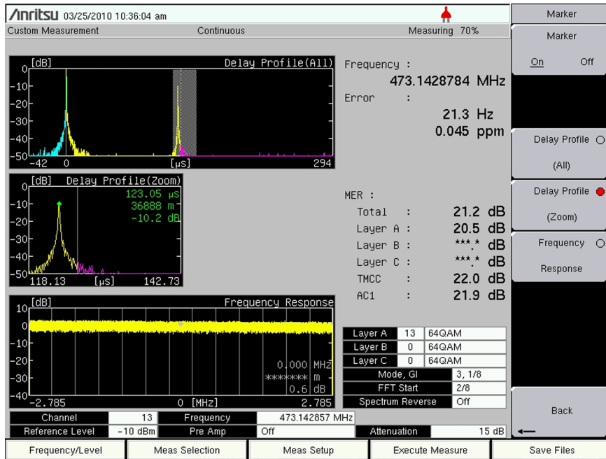
Figure 4-62. Marker Enabled in Delay Profile (Zoom) Graph
