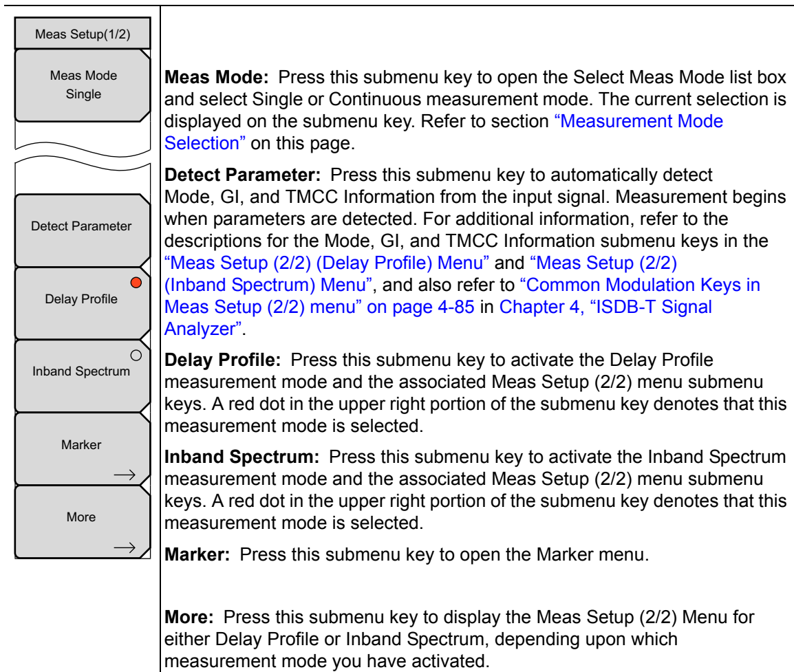
Figure 5-7. Meas Setup (1/2) Menu
