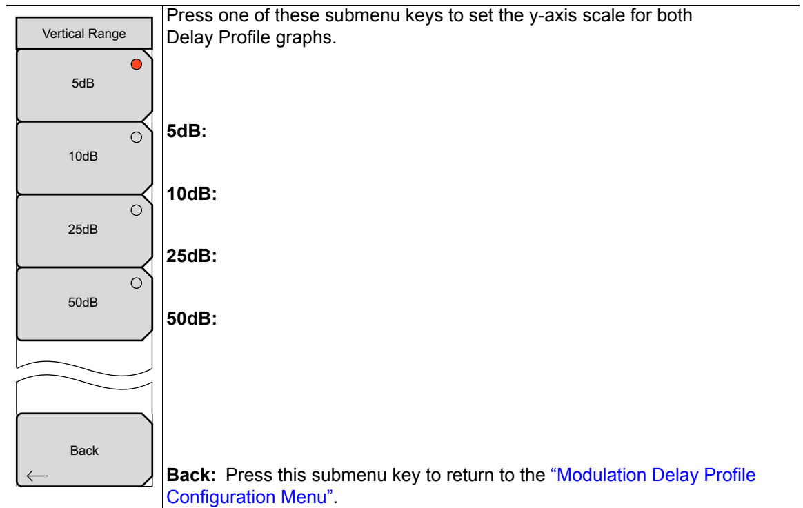
Figure 4-55. Modulation Analysis Delay Profile Vertical Range Menu
