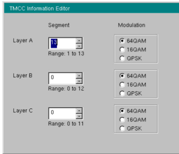
Figure 5-13. TMCC Information Editor Dialog Box
