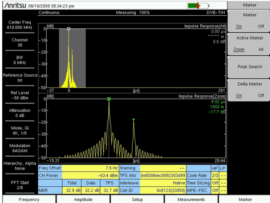
Figure 2-24. Modulation Analysis, Impulse Response View, Delta Marker ON
