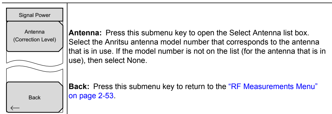
Figure 2-40. Signal Power Menu
