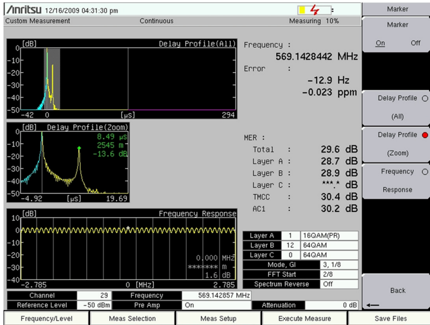
Figure 4-61. Marker Enabled in Delay Profile (Zoom) Graph
