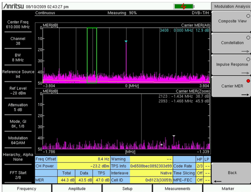
Figure 2-13. Carrier MER
