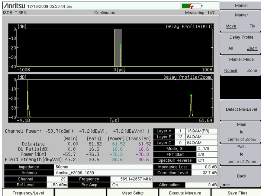
Figure 5-1. SFN Delay Profile Measurement
