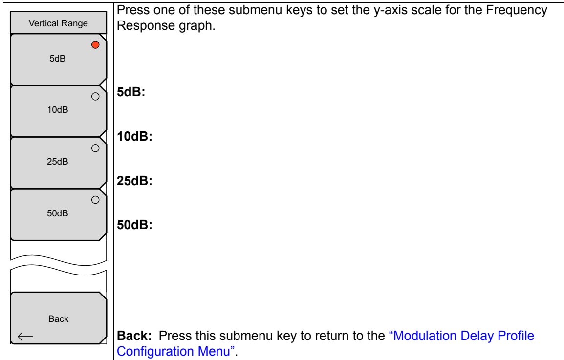
Figure 4-56. Modulation Analysis Delay Profile Freq Response Vertical Range Menu
