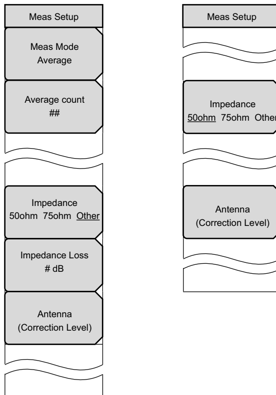
Figure 4-33. Field Strength Measurement Setup Menus for Custom and Easy
