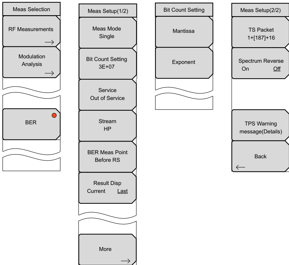
Figure 2-31. DVB-T/H BER Measurements Menu Group (Option 57 Only)
