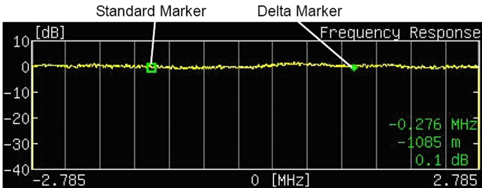
Figure 4-66. Frequency Response Graph with Delta Marker
