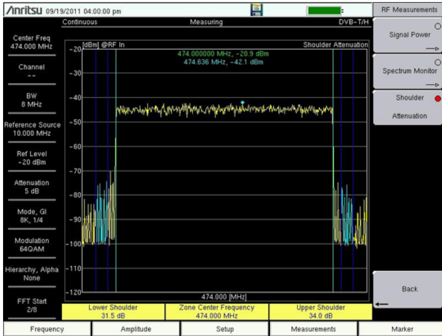
Figure 2-11. Shoulder Attenuation Measurement Screen
