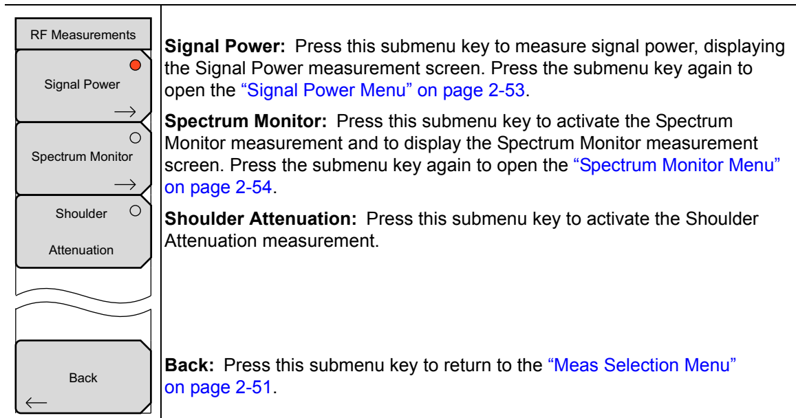
Figure 2-39. RF Measurements Menu
