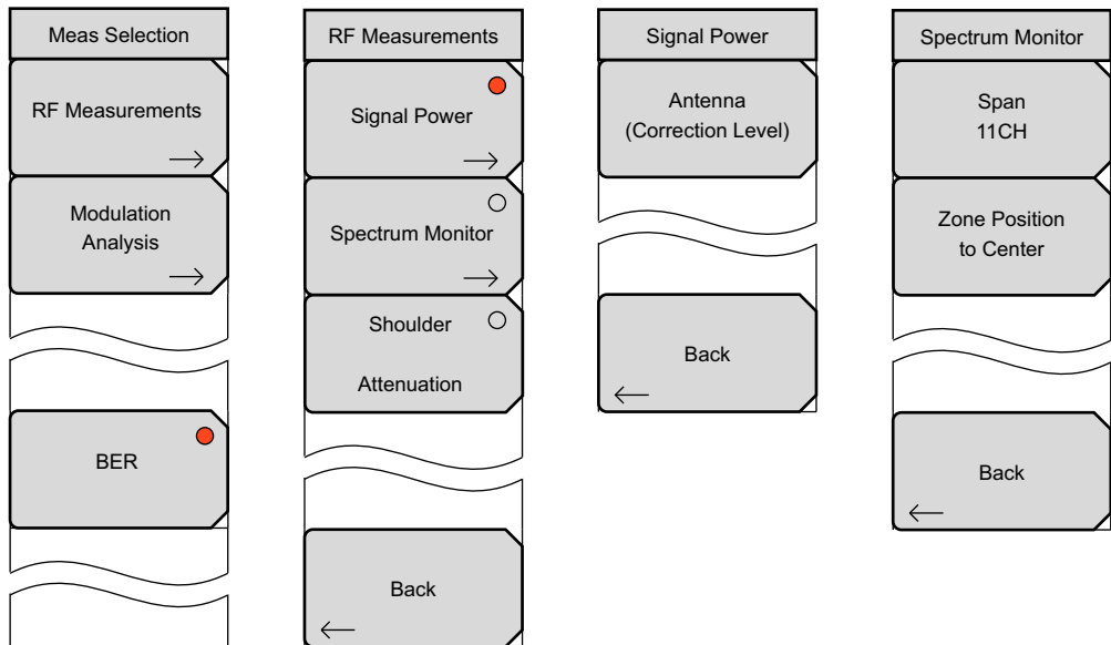
Figure 2-29. DVB-T/H RF Measurements Menu Group
