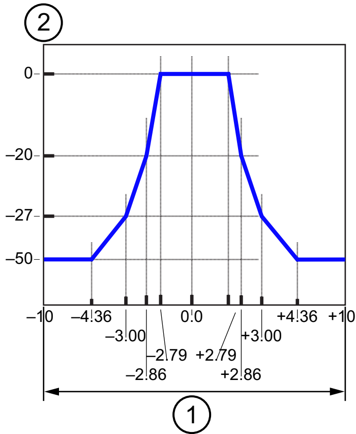
Figure 4-22. Type A Spectrum Mask
