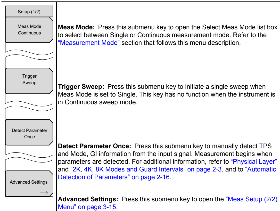
Figure 3-8. Meas Setup (1/2) Menu
