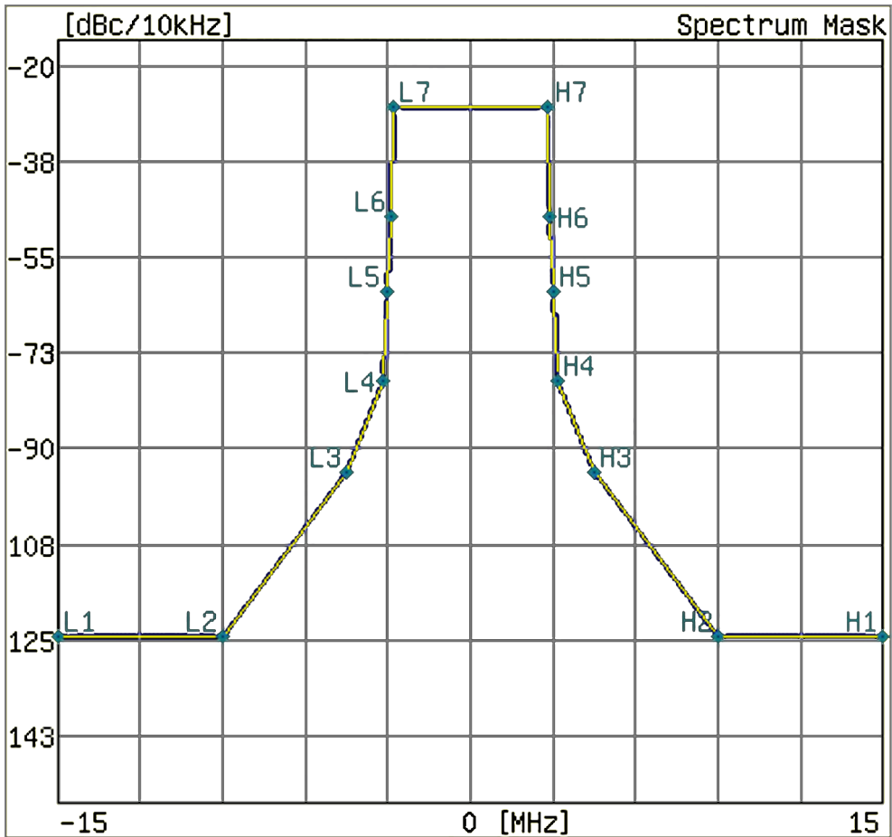
Figure 4-16. Critical Mask for UHF (Brazil) Channel Map
