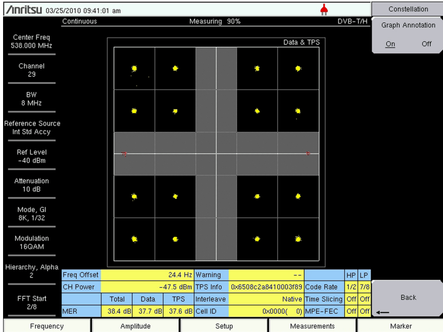
Figure 2-5. 16QAM with Hierarchy set to 2
