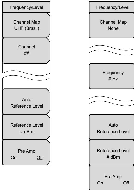
Figure 5-2. Frequency/Level Menus
