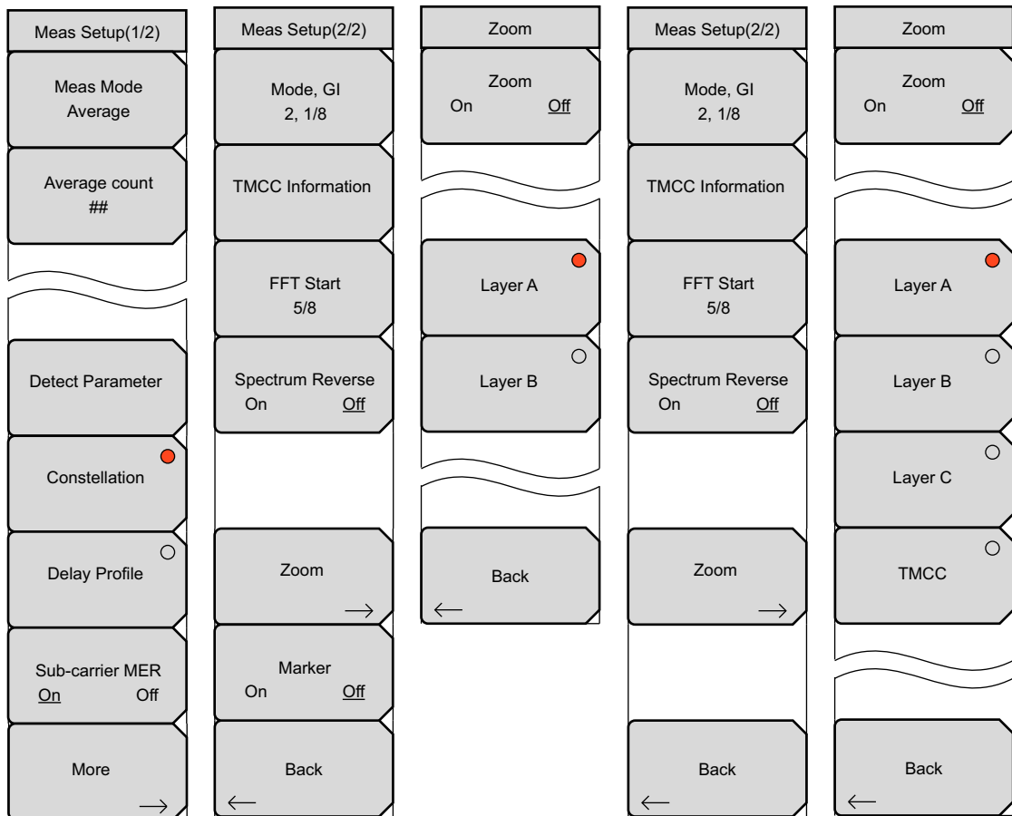
Figure 4-10. Constellation Setup and Zoom Menus
