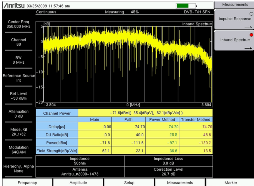
Figure 3-2. Inband Spectrum Measurement
