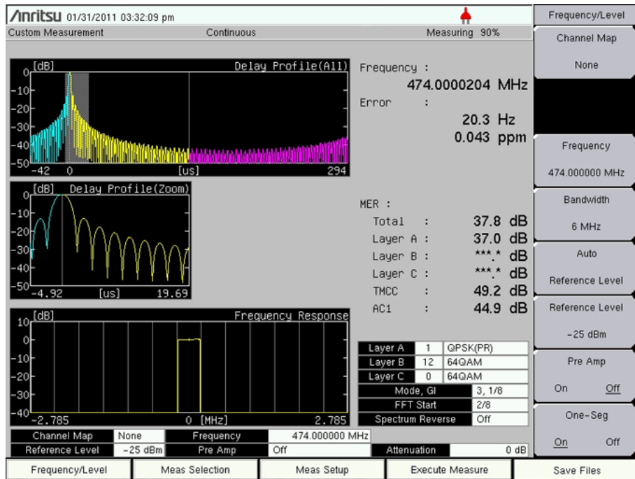
Figure 4-15. Modulation Analysis of Delay Profile, One-Segment
