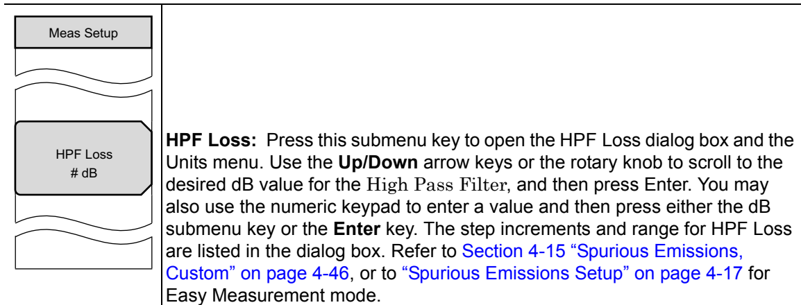
Figure 4-69. Measurement Setup Menu - Spurious Emissions Measurement (Custom and Easy)
