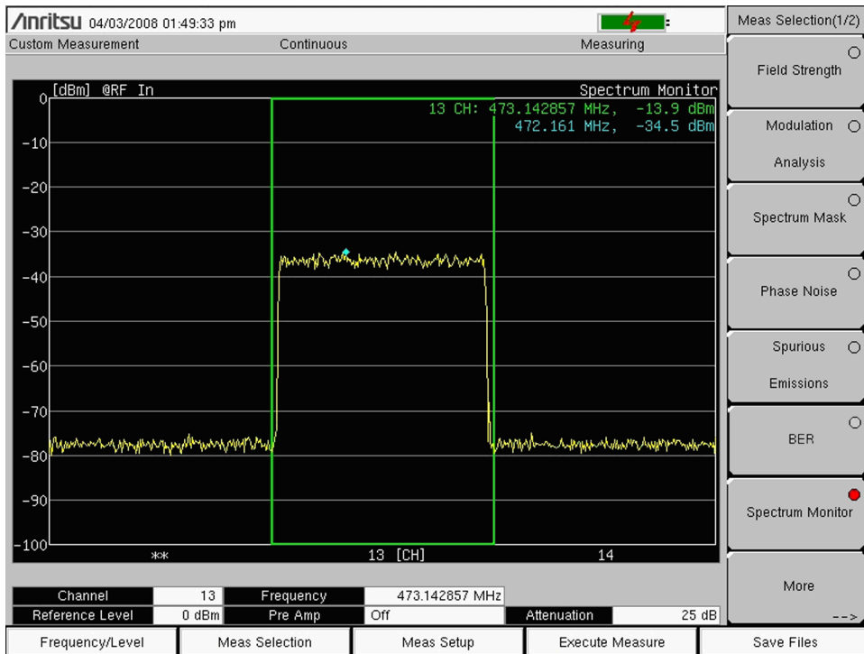
Figure 4-26. Spectrum Monitor Display
