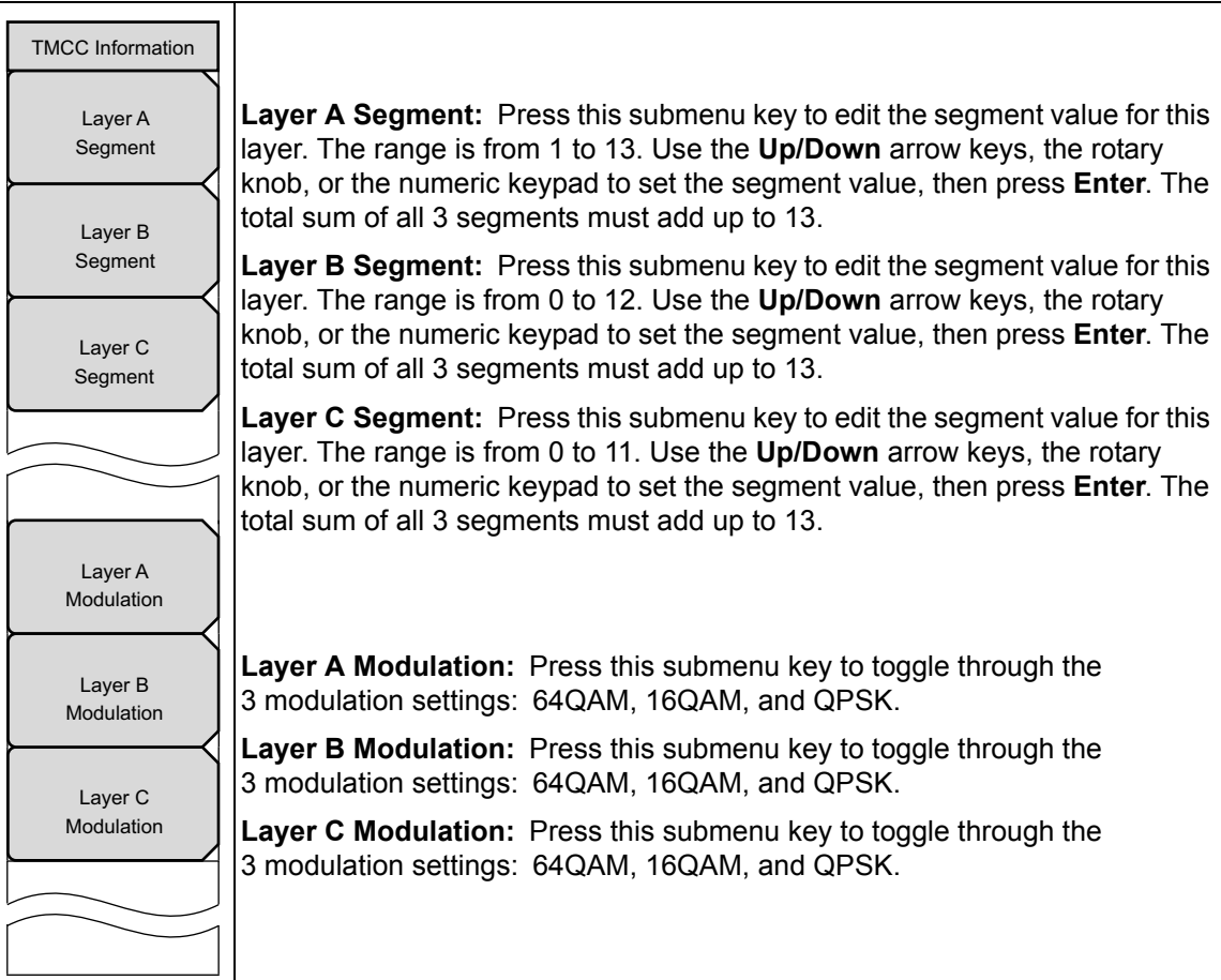
Figure 5-12. TMCC Information Menu
