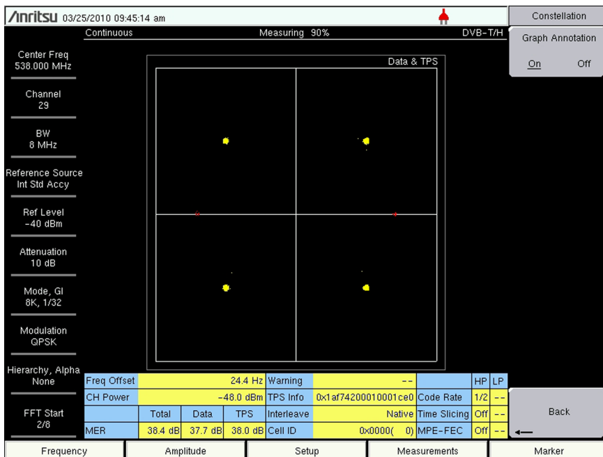
Figure 2-2. QPSK with Hierarchy set to None
