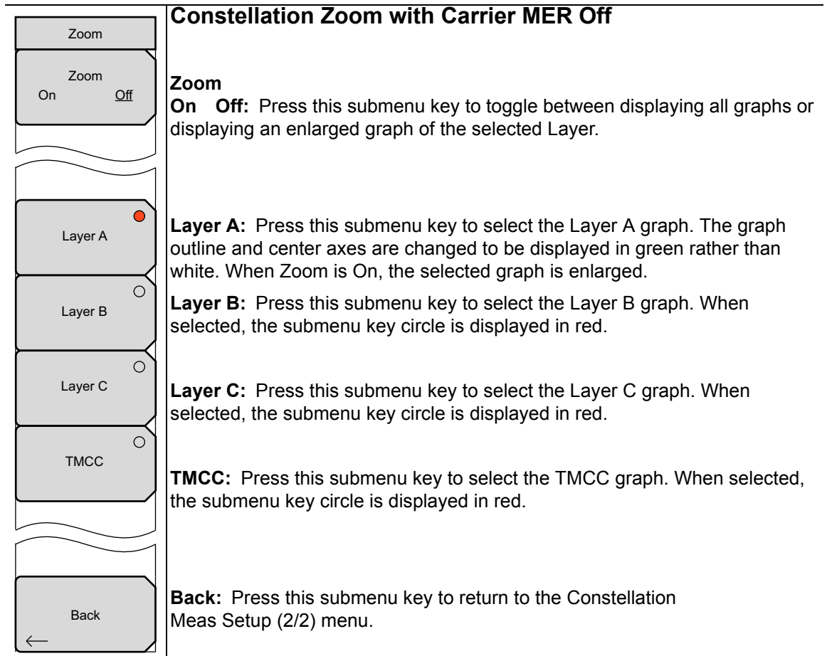
Figure 4-53. Modulation Analysis Constellation Zoom Menu (Sub-carrier MER Off)
