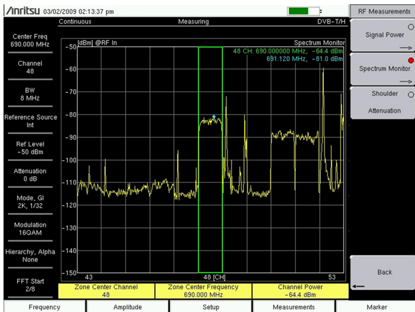
Figure 2-10. Spectrum Monitor Measurement Screen
