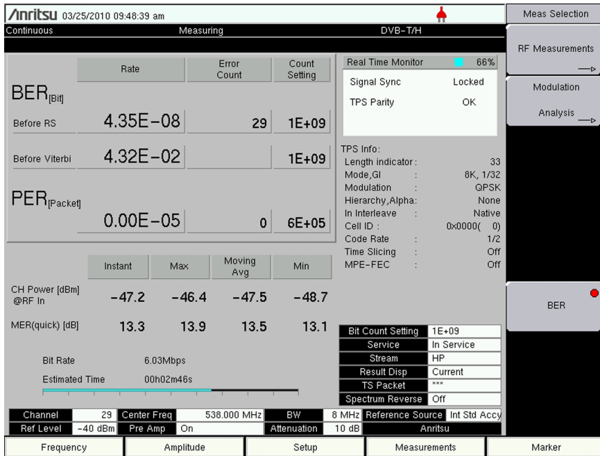
Figure 2-14. Bit Error Rate (BER) Measurements
