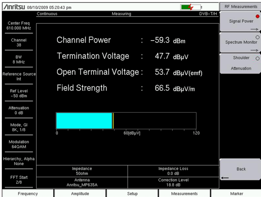
Figure 2-9. Signal Power Measurement Screen
