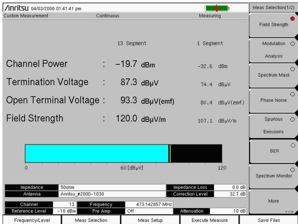
Figure 4-8. Field Strength Measurement Screen
