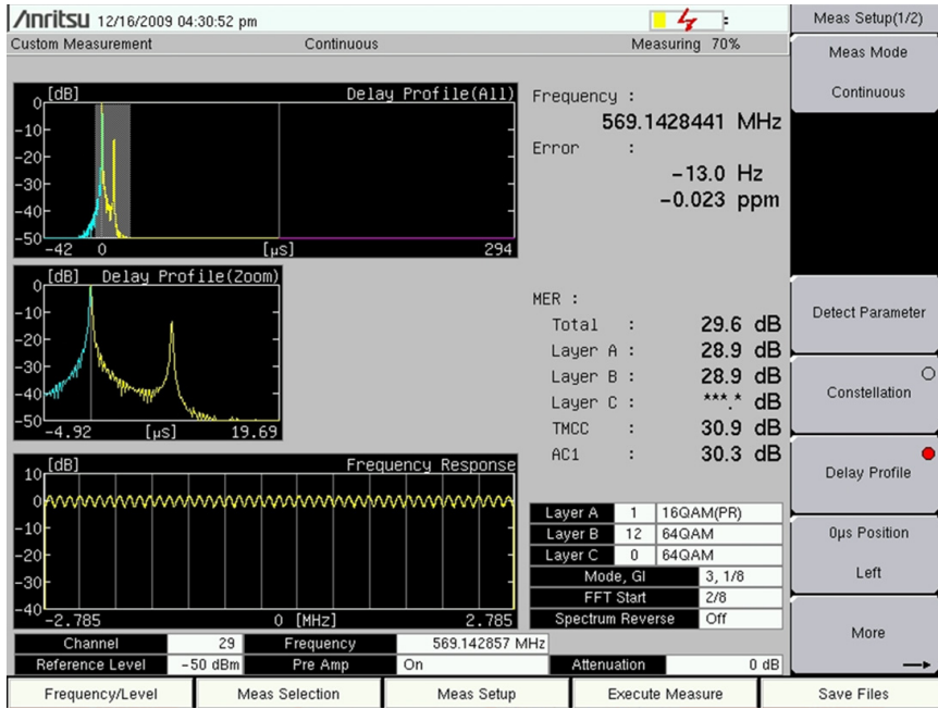
Figure 4-60. Modulation Analysis – Delay Profile Measurement Display
