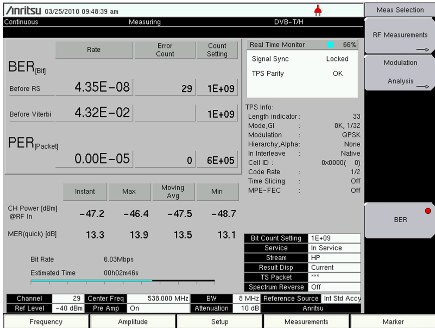
Figure 2-27. Bit Error Rate (BER) Measurements
