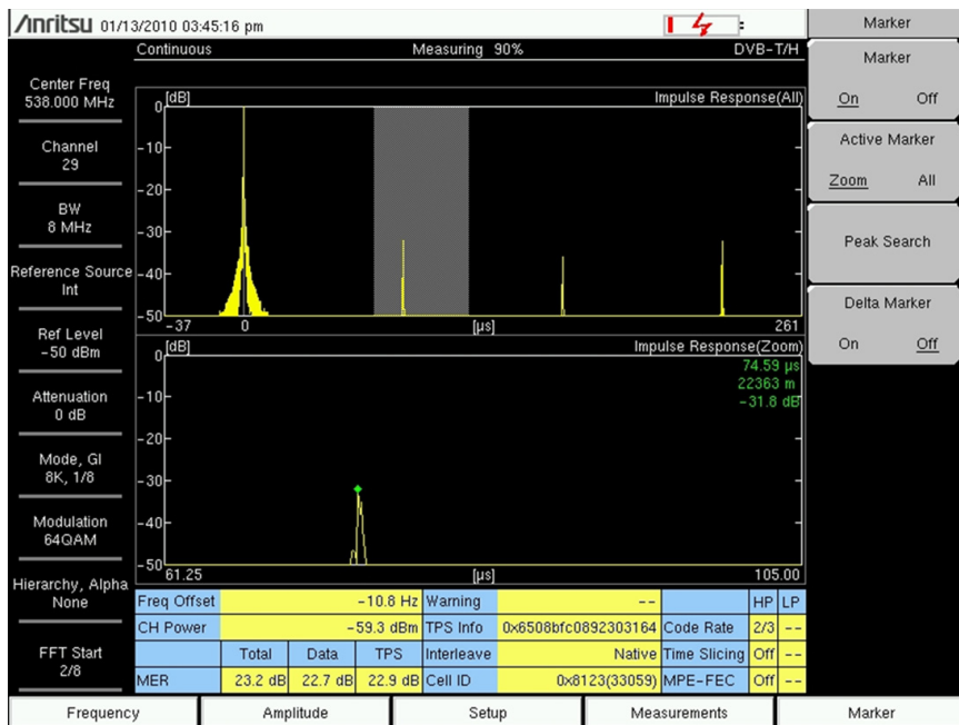
Figure 2-25. Modulation Analysis, Impulse Response View, Delta Marker OFF
