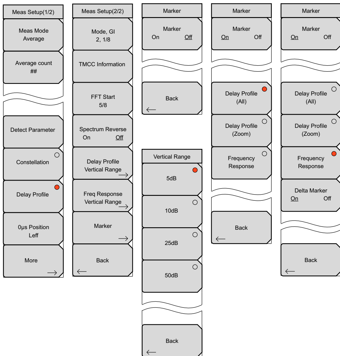
Figure 4-12. Delay Profile Setup and Marker Menus
