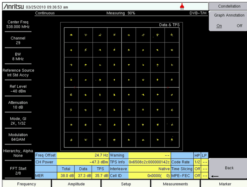
Figure 2-4. 64QAM with Hierarchy set to None
