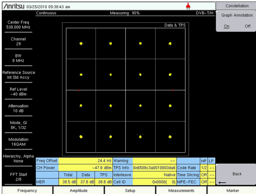
Figure 2-3. 16QAM with Hierarchy set to None
