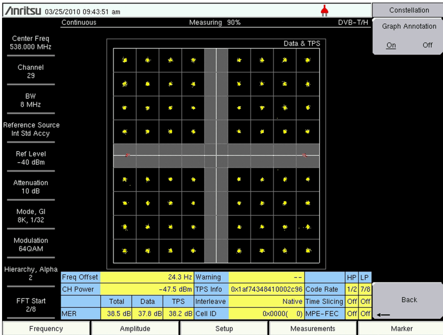
Figure 2-7. 64QAM with Hierarchy set to 2
