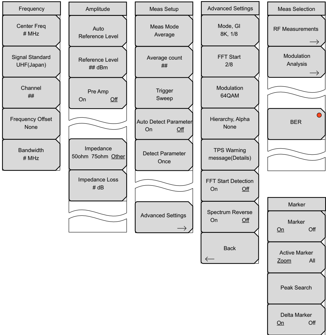
Figure 2-28. DVB-T/H Main Menu Group
