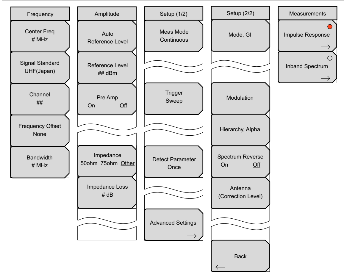
Figure 3-3. Main Menu Group
