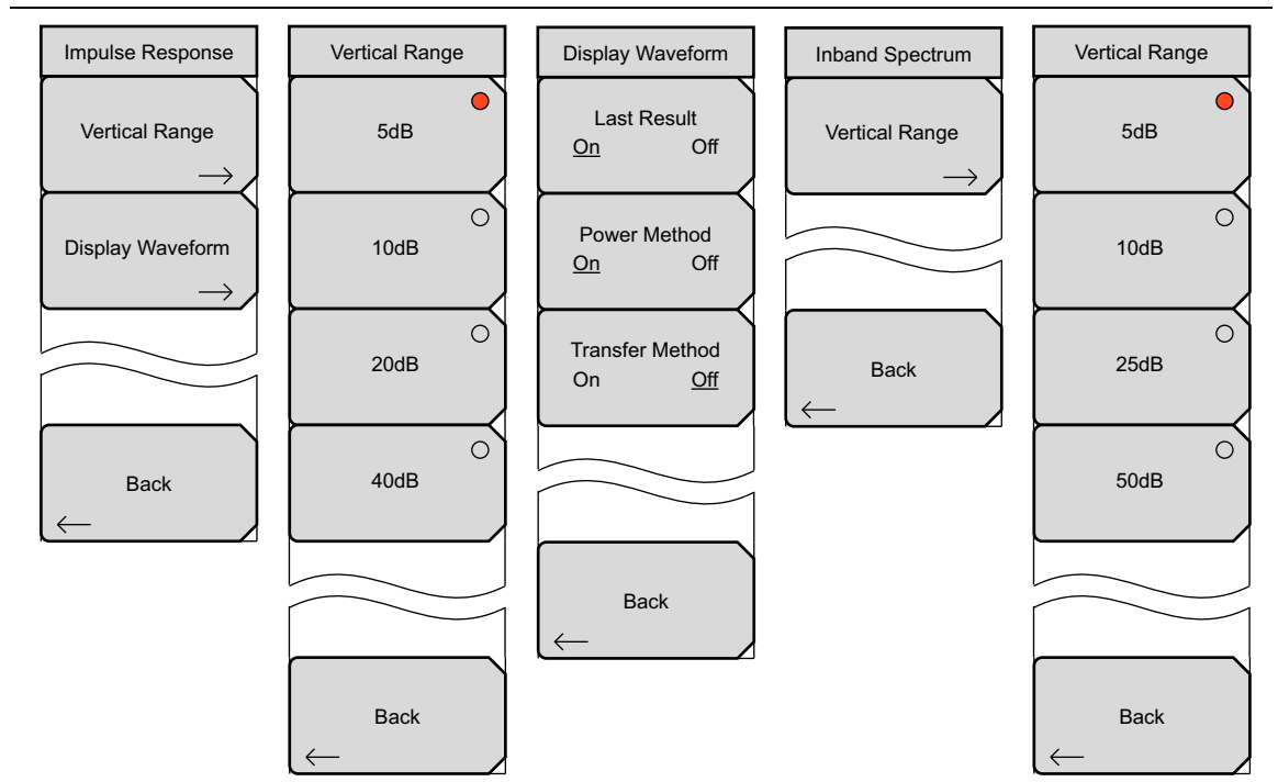
Figure 3-4. Measurements Menu Group
