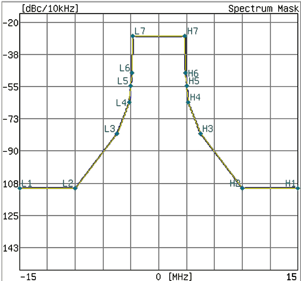
Figure 4-18. Noncritical Mask for UHF (Brazil) Channel Map
