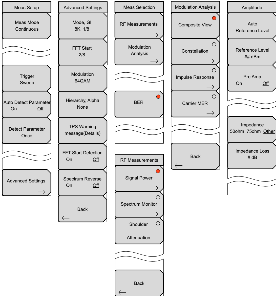
Figure 2-15. Measurement Setup and Selection Menus
