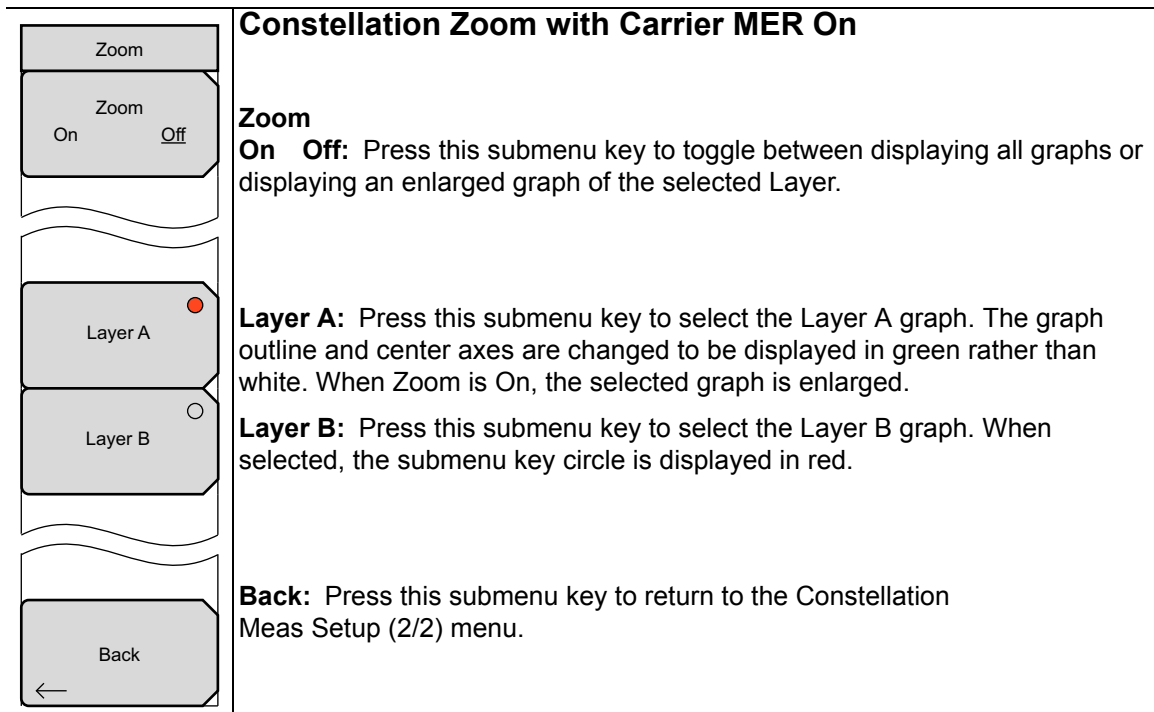
Figure 4-52. Modulation Analysis Constellation Zoom Menu (Sub-carrier MER On)
