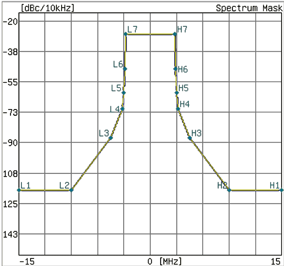
Figure 4-17. Subcritical Mask for UHF (Brazil) Channel Map
