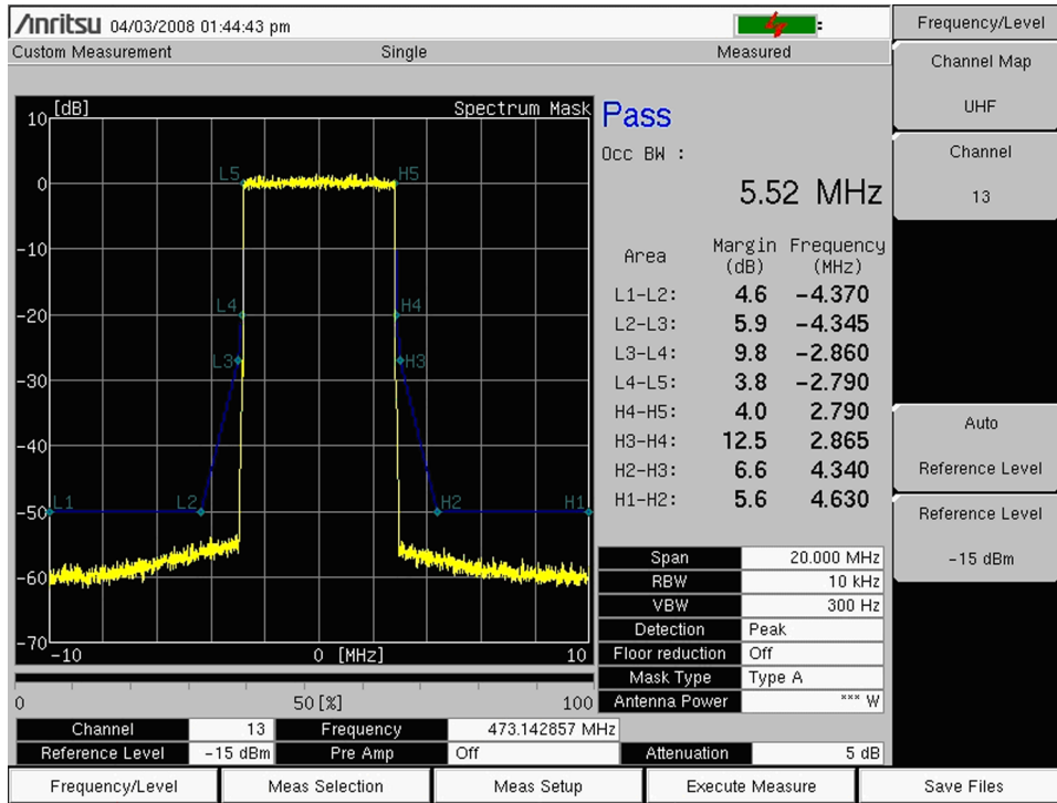
Figure 4-21. Transmitter Spectrum Mask
