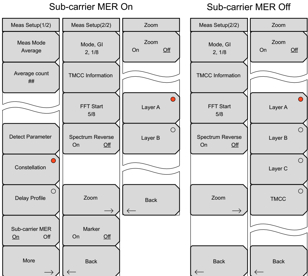
Figure 4-35. Constellation Setup and Zoom Menus — Custom
