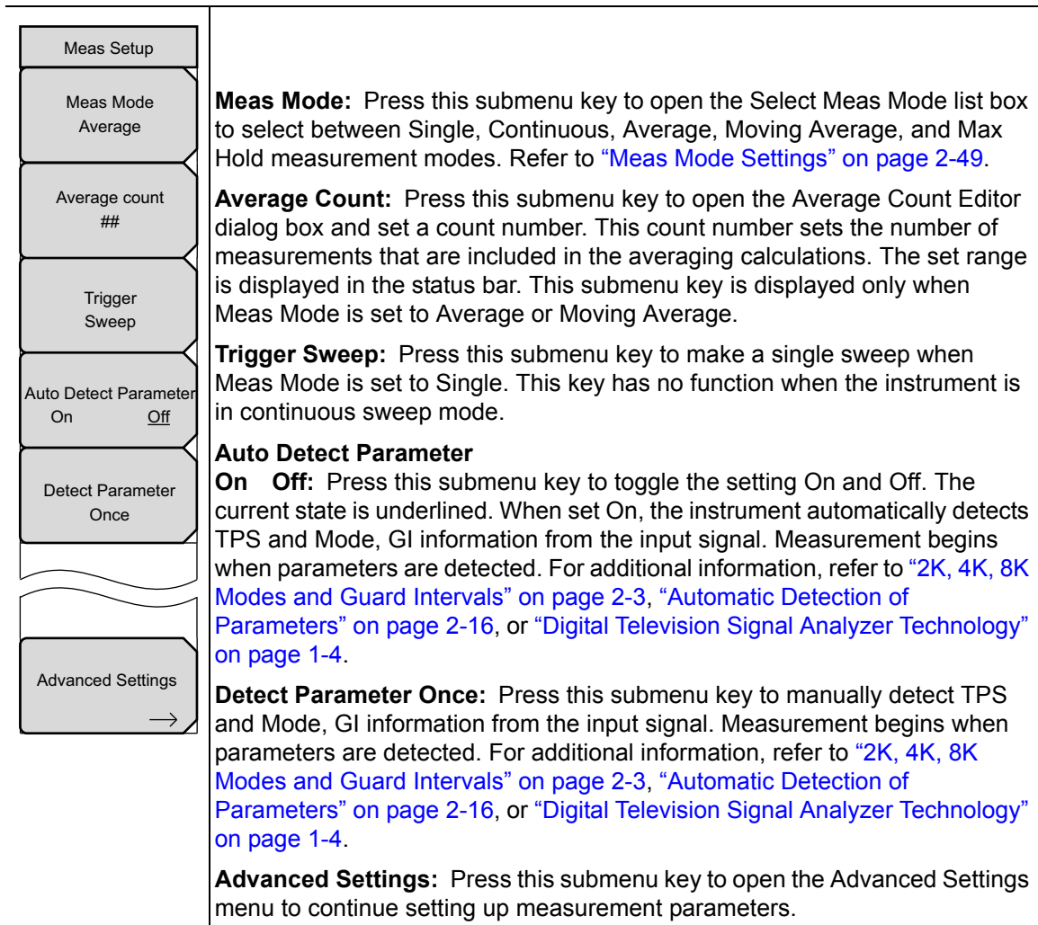
Figure 2-35. Meas Setup Menu
