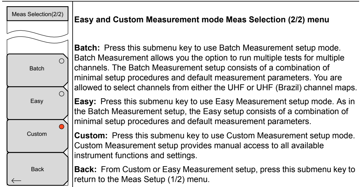
Figure 4-39. Measurement Selection (2/2) Menu (Custom and Easy)
