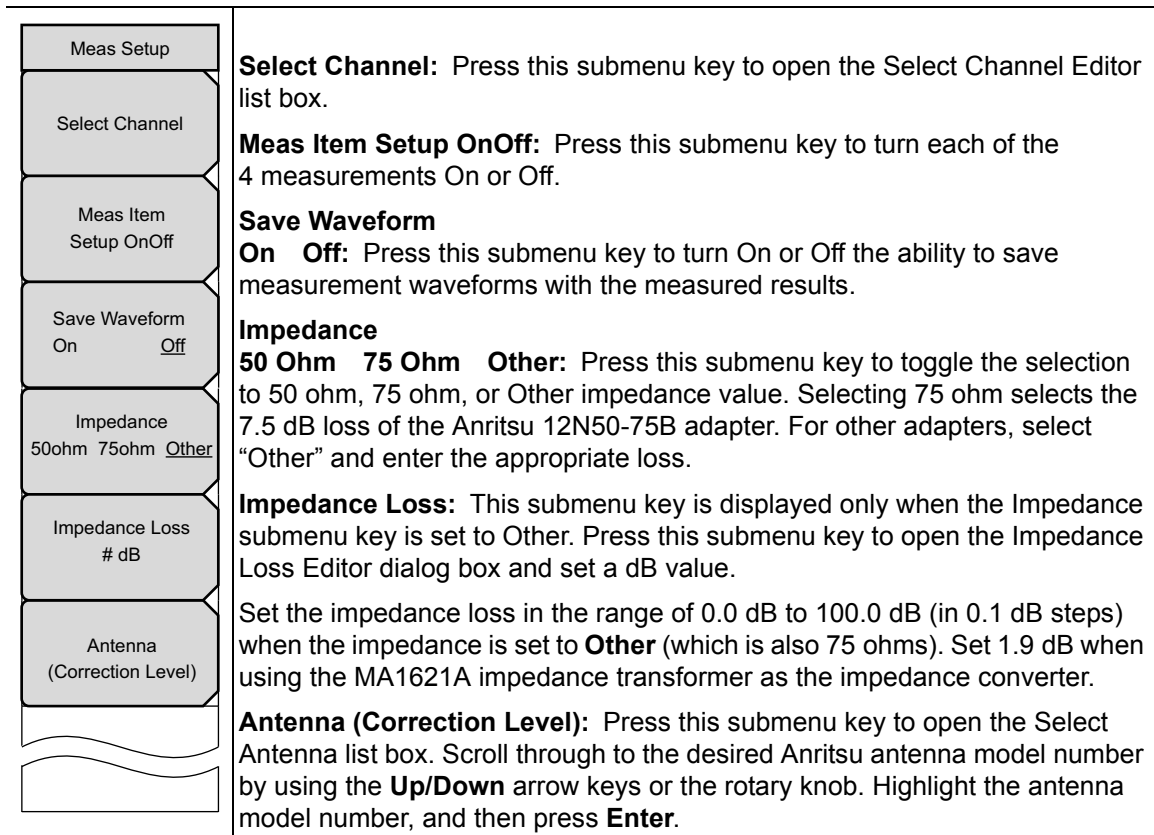
Figure 4-5. Batch Measurement Setup Menu
