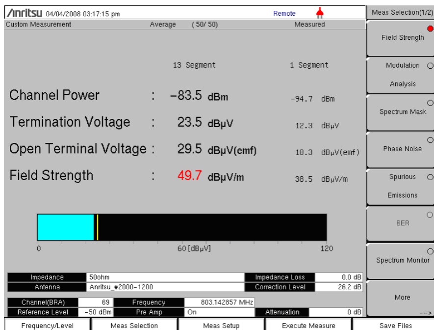
Figure 4-3. Measurement Screen and Meas Selection (1/2) Menu
