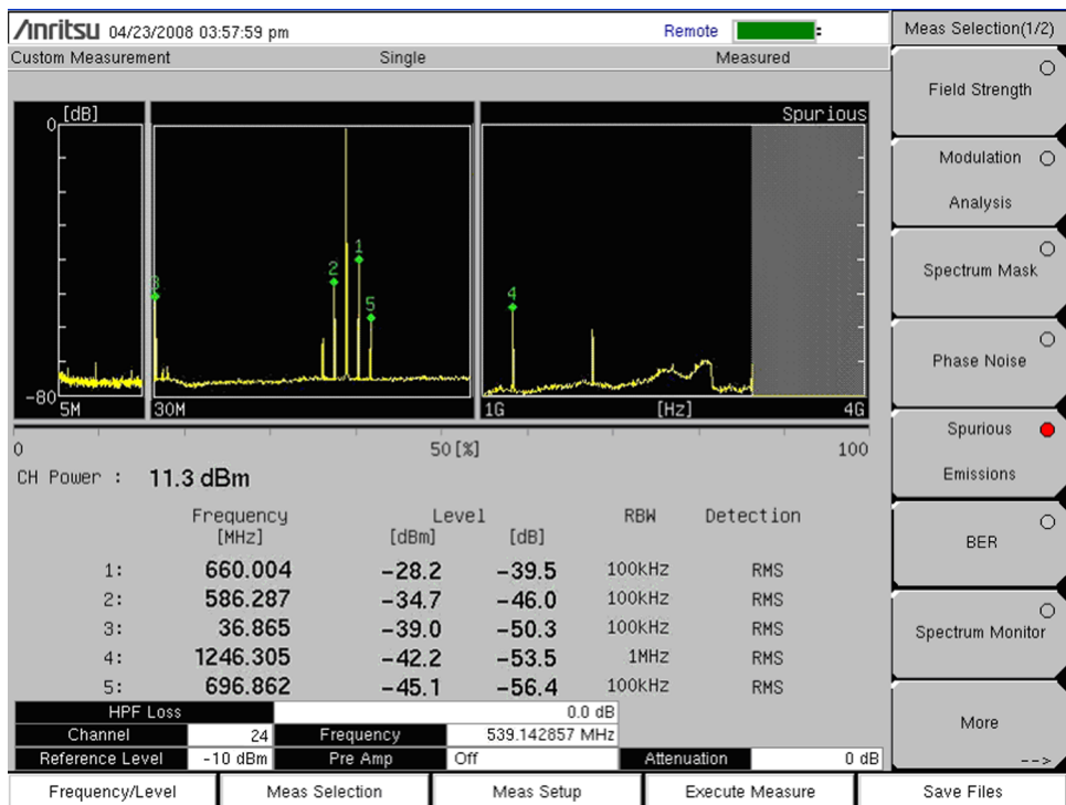
Figure 4-24. Spurious Emissions Measurement
