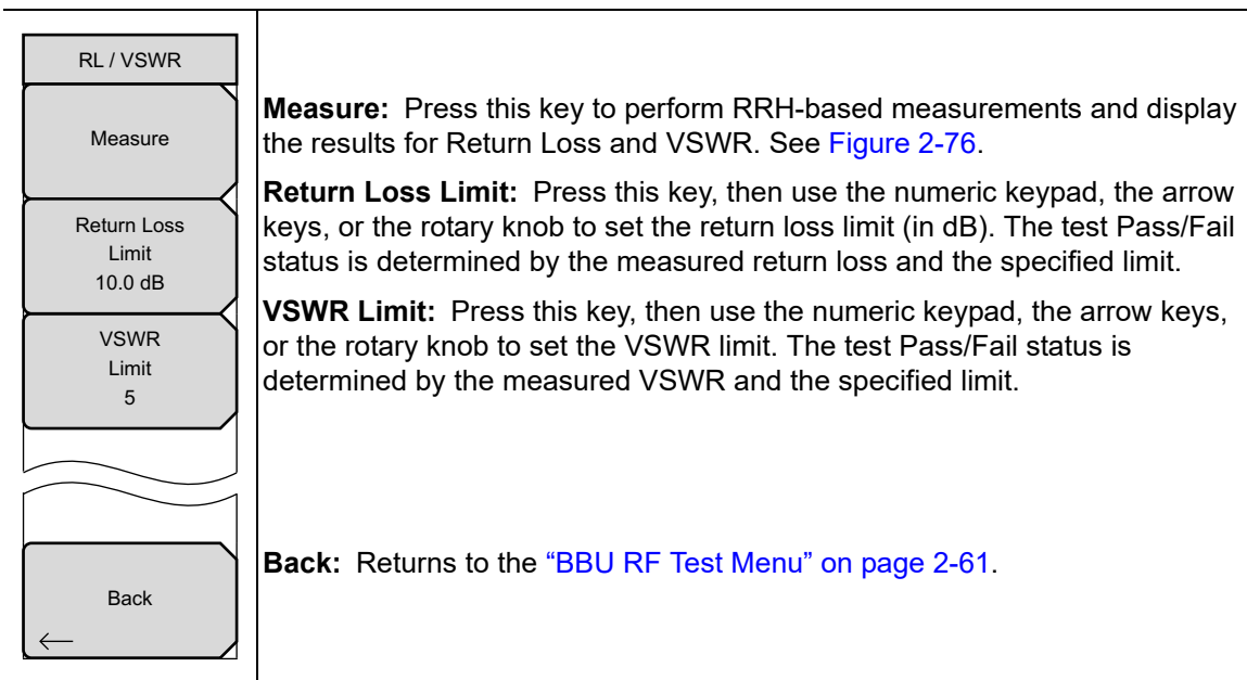
Figure 2-75. RL/VSWR Menu
