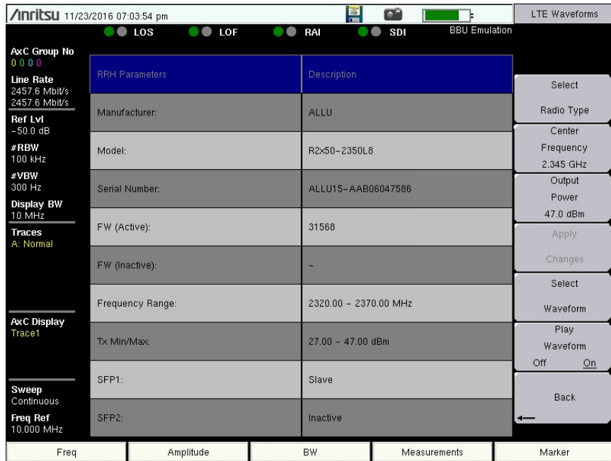
Figure 2-30. Play Waveform
