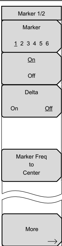
Figure 2-99. Marker 1/2 Menu
