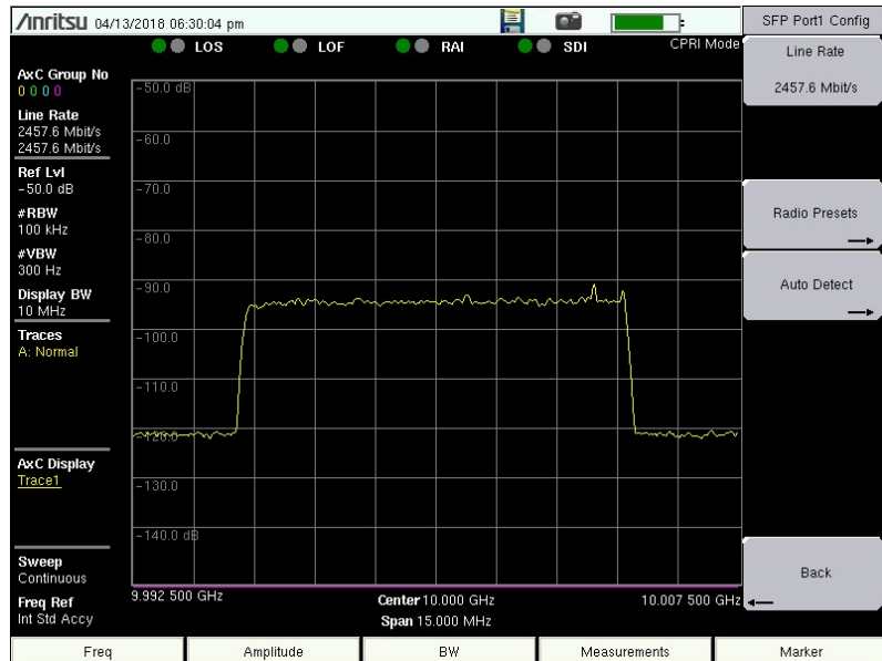
Figure 2-9. Sample Spectrum Display
