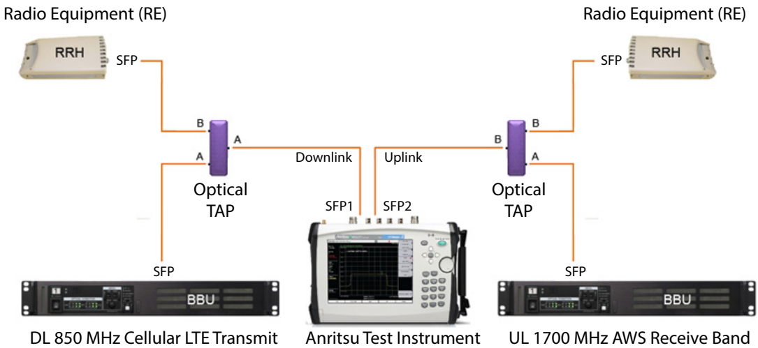
Figure 2-33. 2nd Harmonic Test Instrument Connection
