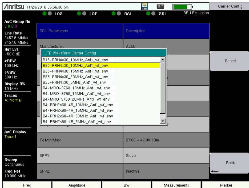
Figure 2-27. LTE Waveform Carrier Configuration
