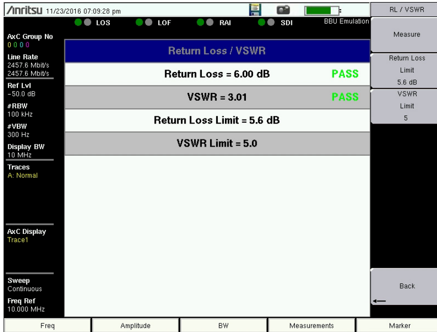
Figure 2-31. Return Loss/VSWR Measurement Results
