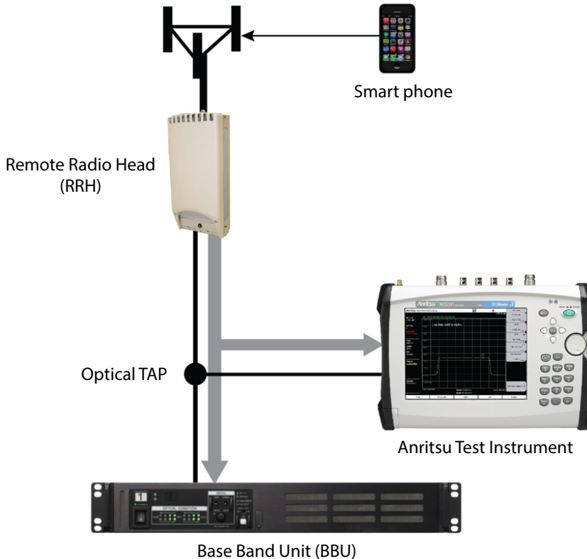
Figure 2-1. Connection Configuration for CPRI LTE RF Testing with Anritsu Test Instrument
