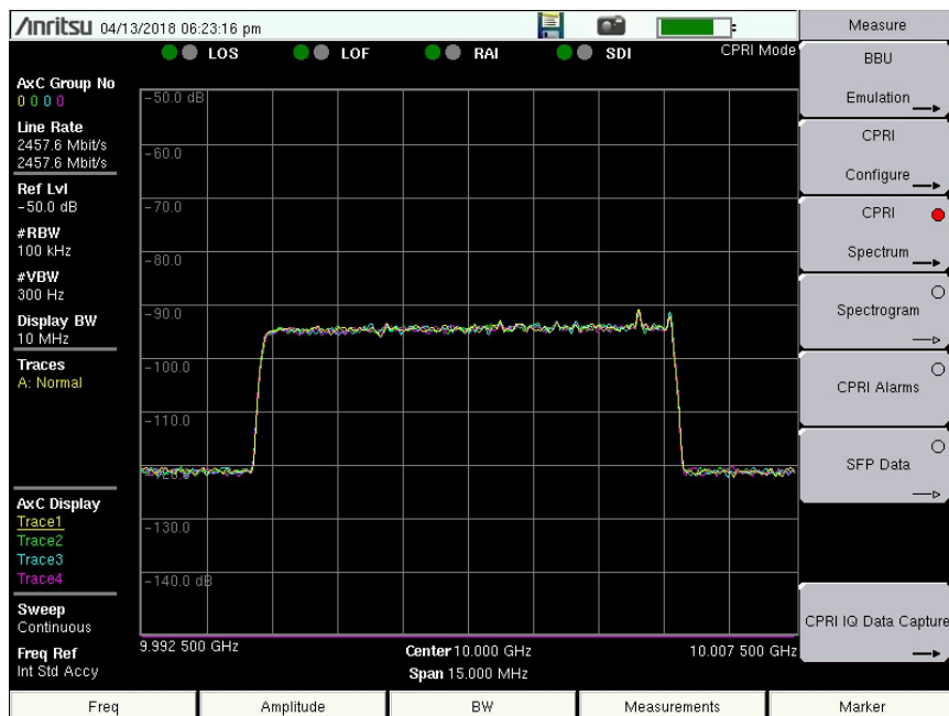
Figure 2-5. CPRI Spectrum Display
