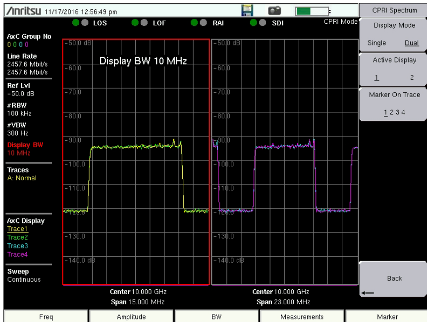
Figure 2-87. Spectrum Dual Display
