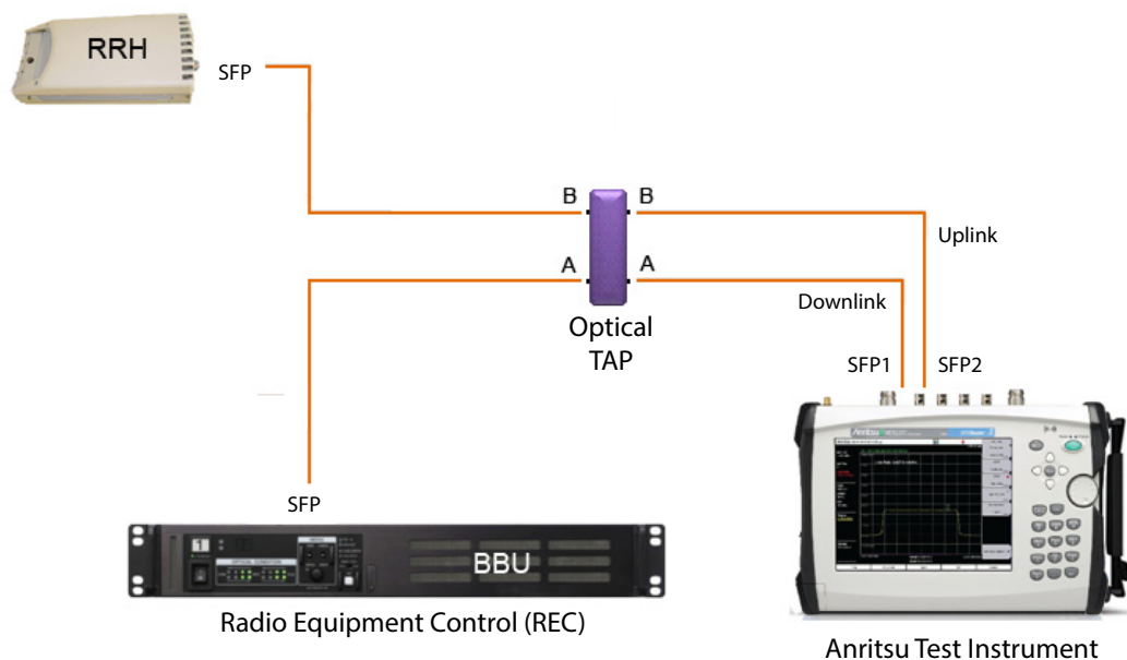
Figure 2-32. Self-PIM Interference Test Instrument Connection
