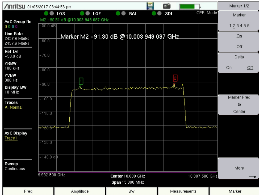
Figure 2-101.Active Marker M2
