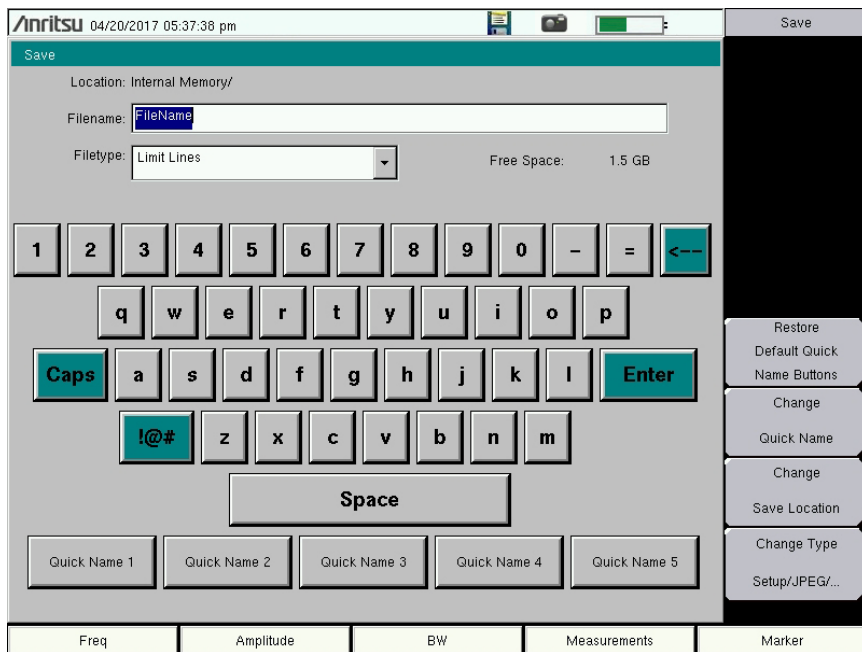
Figure 2-115. Save Dialog
