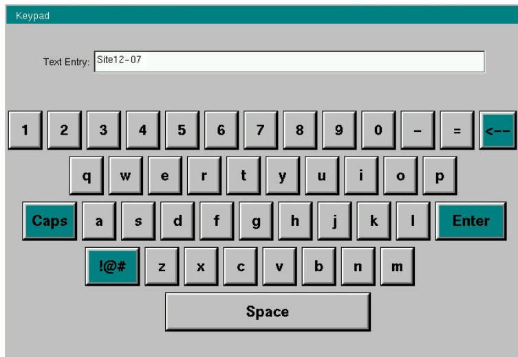
Figure 2-98. Virtual Keyboard
