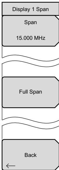
Figure 2-54. Span Menu
