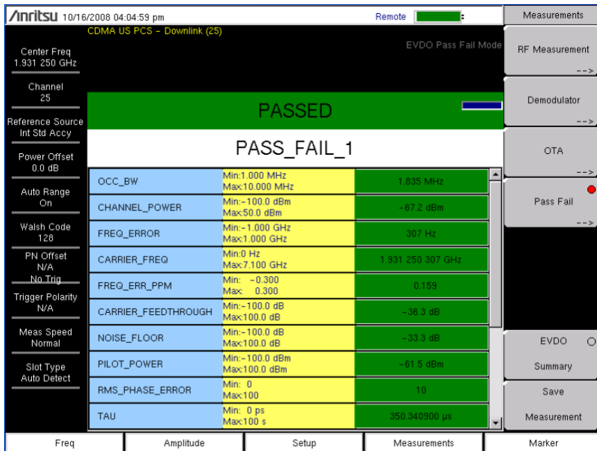
Figure 3-12. Pass Fail Measurement
