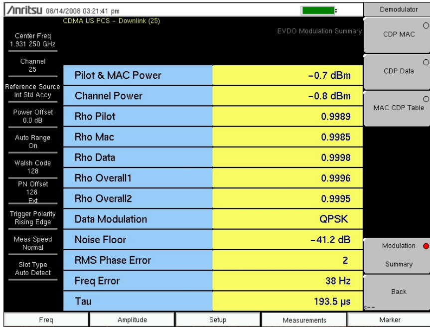
Figure 3-9. EVDO Modulation Summary
