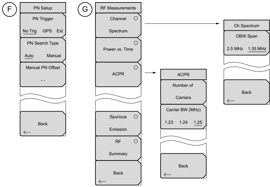
Figure 3-14. EVDO Menu Layout (1 of 2)
