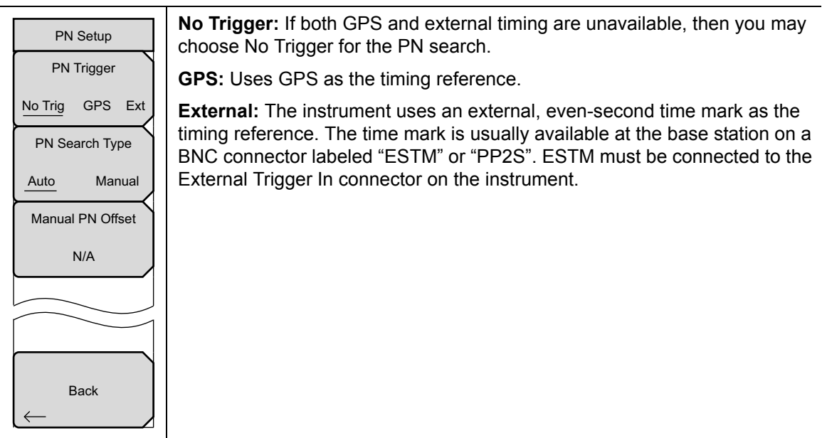
Figure 3-1. PN Setup
