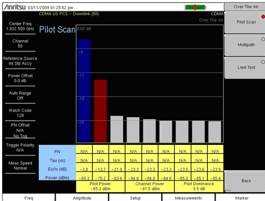
Figure 2-8. Over-The-Air Pilot Scan Measurement
