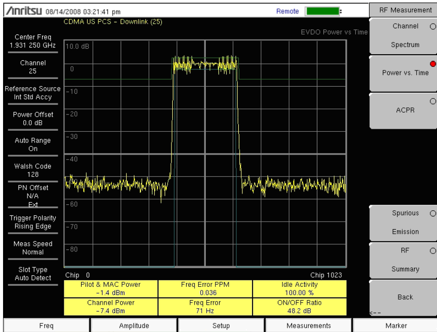
Figure 3-3. EVDO Power vs. Time
