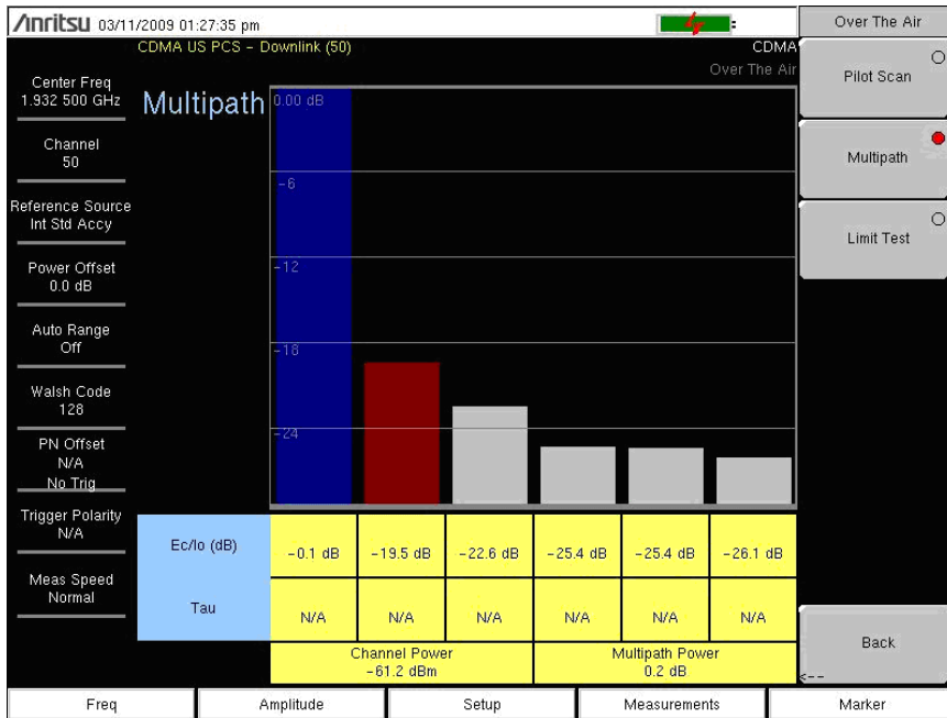
Figure 2-9. Over-The-Air Pilot Multipath Measurement
