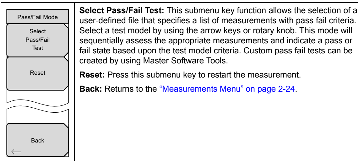
Figure 2-25. CDMA Pass Fail Mode Menu
