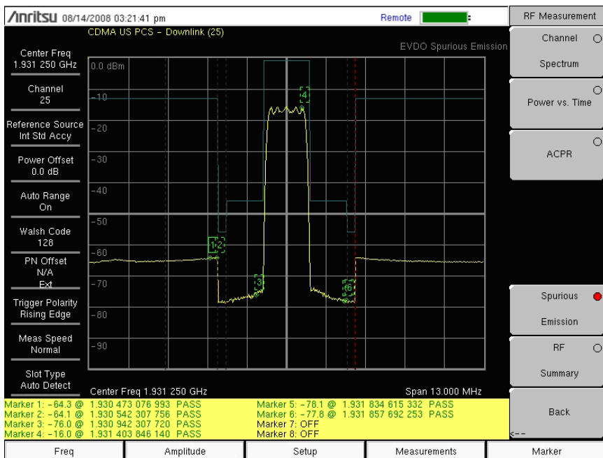
Figure 3-5. EVDO Spurious Emission
