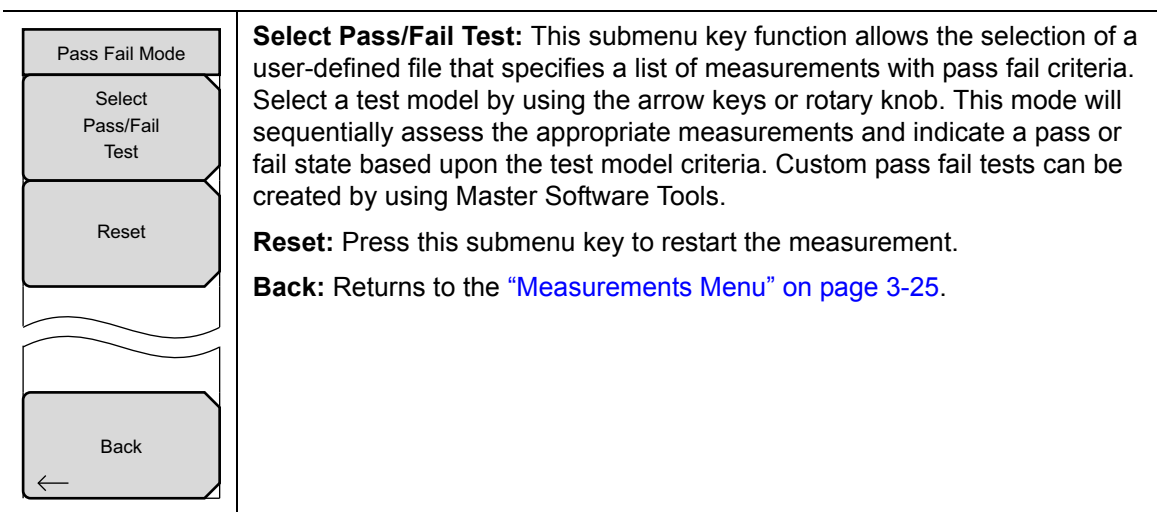
Figure 3-28. EVDO Pass Fail Mode Menu
