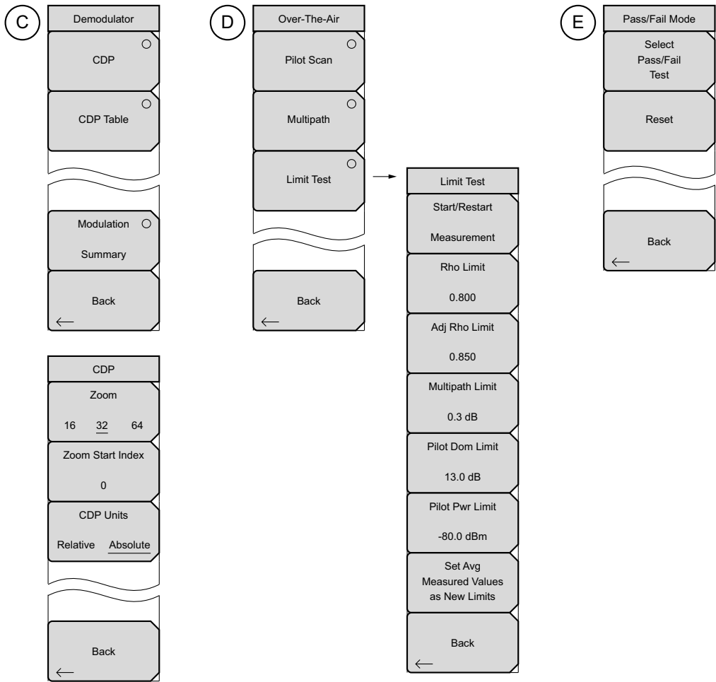
Figure 2-13. CDMA Menu Layout (2 of 2)
