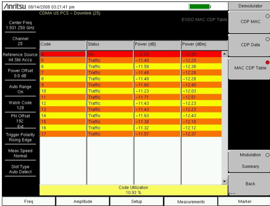
Figure 3-8. EVDO MAC CDP Table
