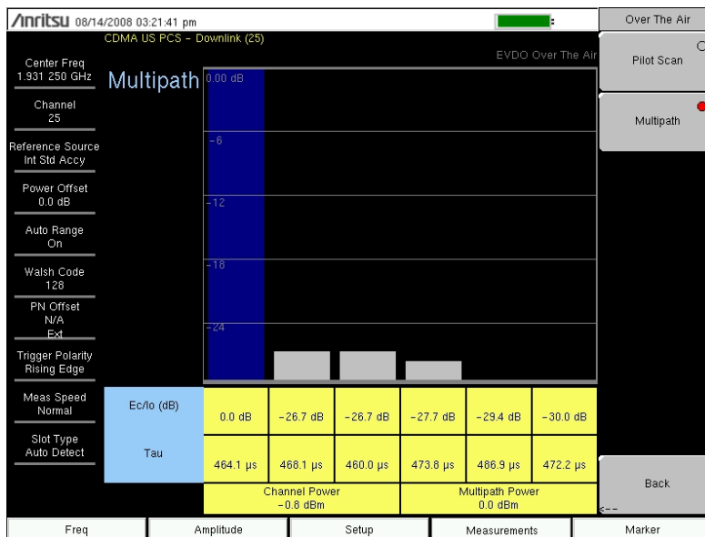
Figure 3-11. EVDO OTA Multipath
