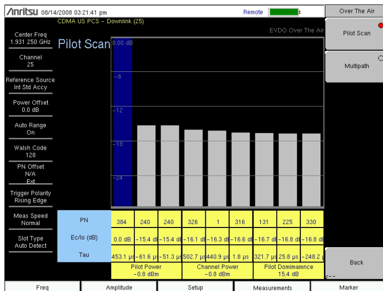
Figure 3-10. EVDO OTA Pilot Scan
