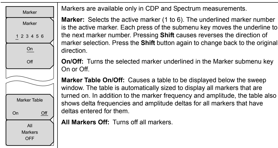
Figure 2-26. CDMA Marker Menu
