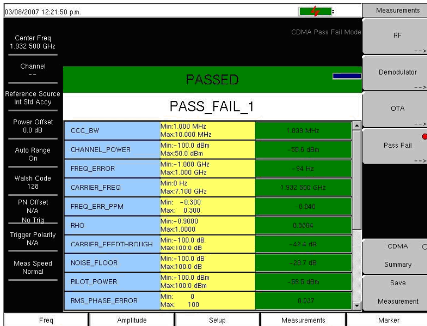
Figure 2-11. Pass Fail Measurement
