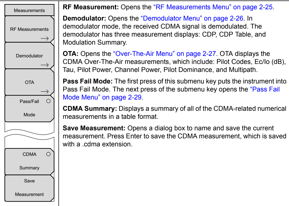
Figure 2-18. CDMA Measurements Menu
