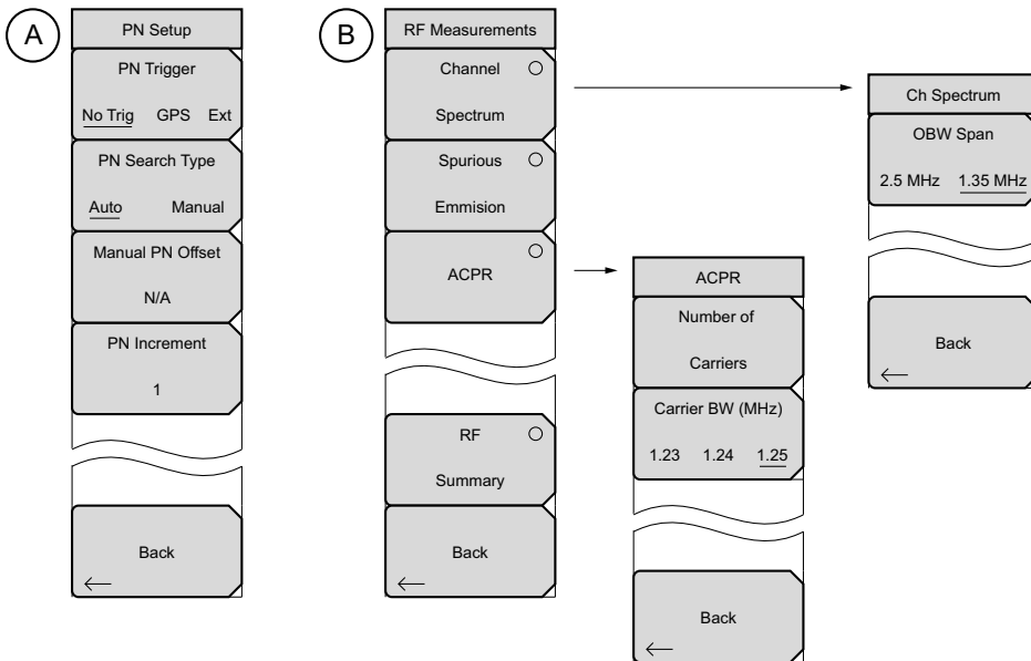
Figure 2-12. CDMA Menu Layout (1 of 2)
