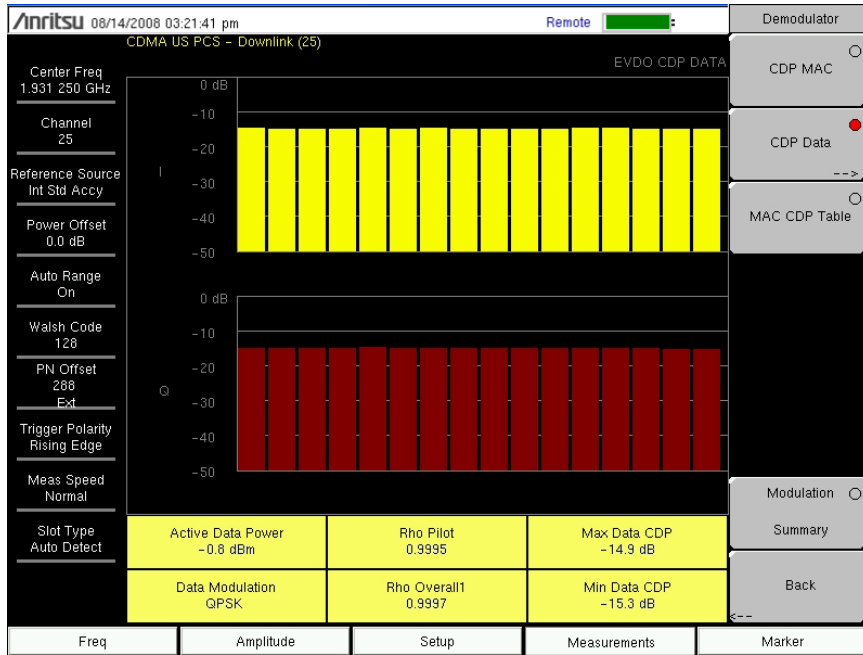
Figure 3-7. EVDO CDP Data
