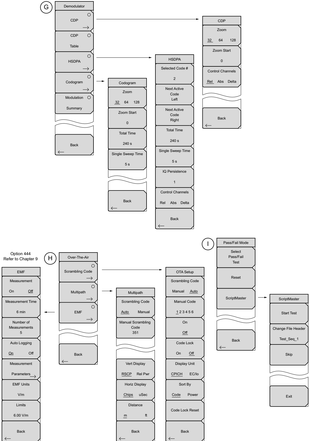
Figure 3-15. W-CDMA/HSDPA Menu Layout (2 of 2)
