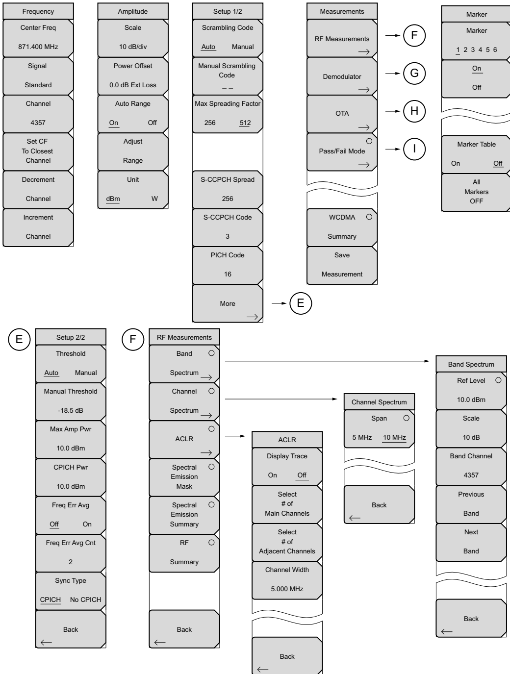
Figure 3-14. W-CDMA/HSDPA Menu Layout (1 of 2)
