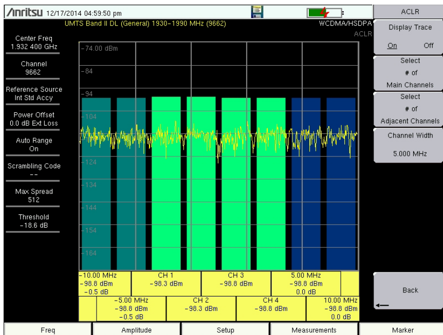
Figure 3-4. ACLR Multi-channel Measurement
