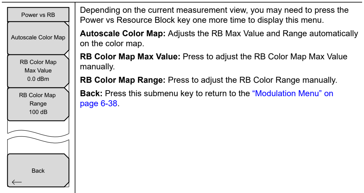
Figure 6-34. TD-LTE Power vs. Resource Block Menu
