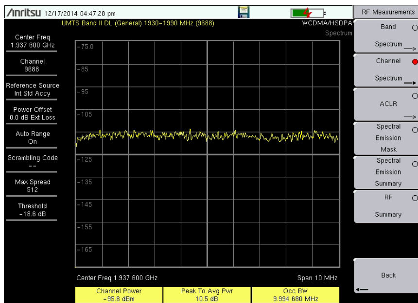
Figure 3-2. Channel Spectrum
