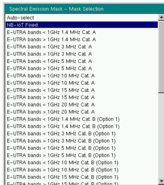
Figure 8-4. Spectral Emission Mask List Box
