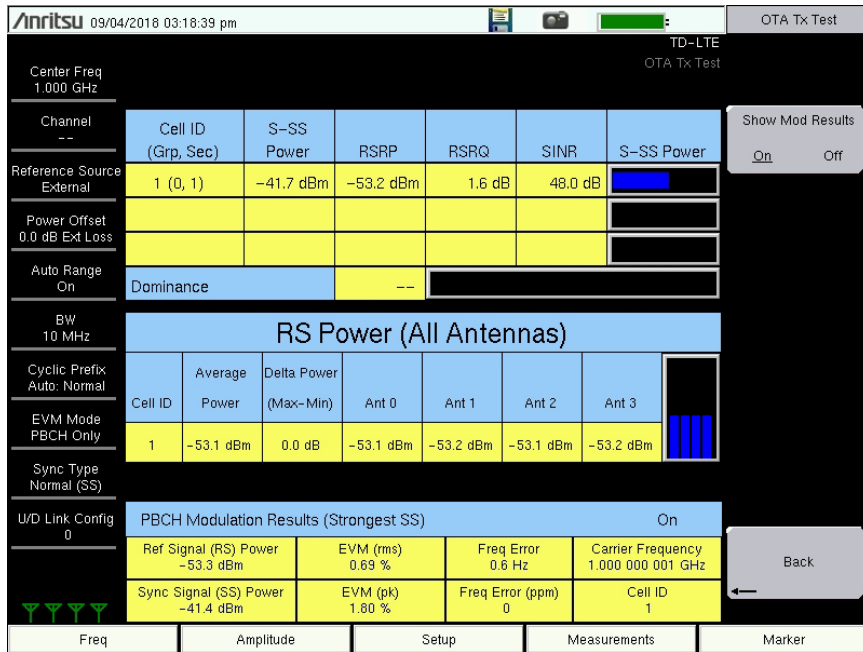
Figure 6-14. Over-the-Air Tx Test Measurement
