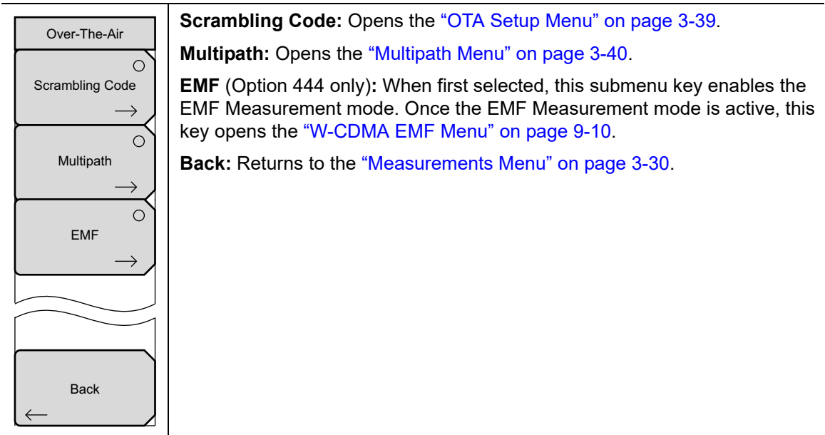
Figure 3-29. W-CDMA/HSDPA Over-The-Air Menu
