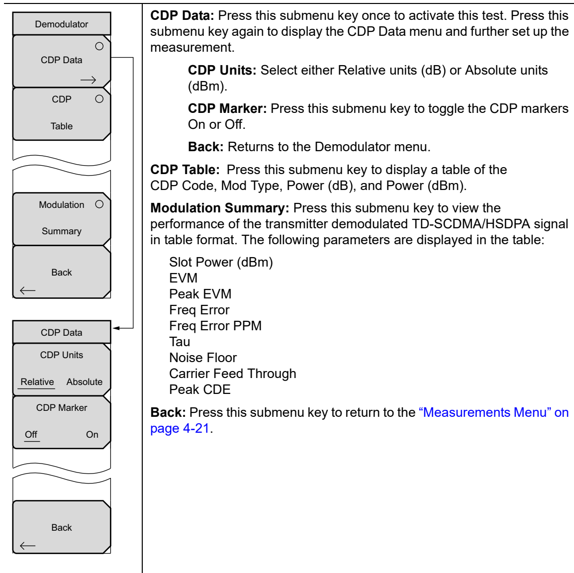
Figure 4-23. TD-SCDMA/HSDPA Demodulator Menu
