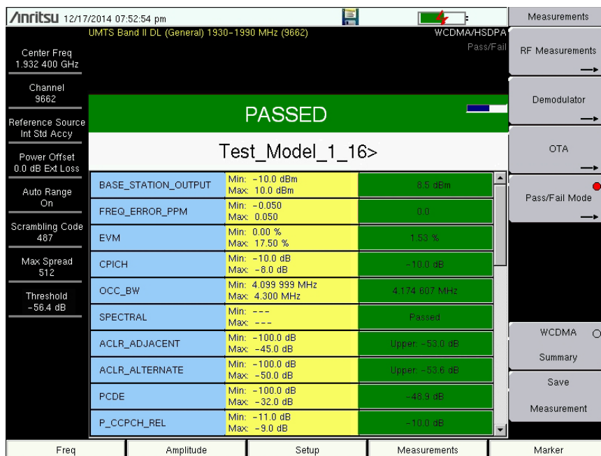
Figure 3-13. Pass/Fail Mode
