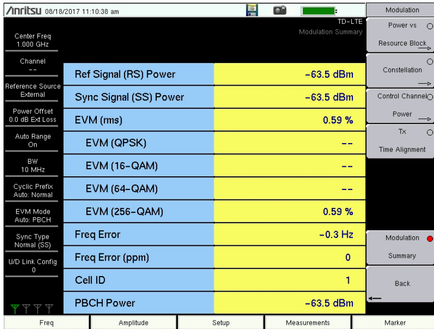
Figure 6-12. Modulation Summary
