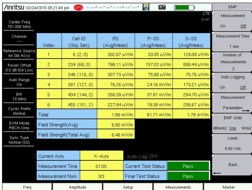
Figure 9-7. LTE EMF Measurement Results
