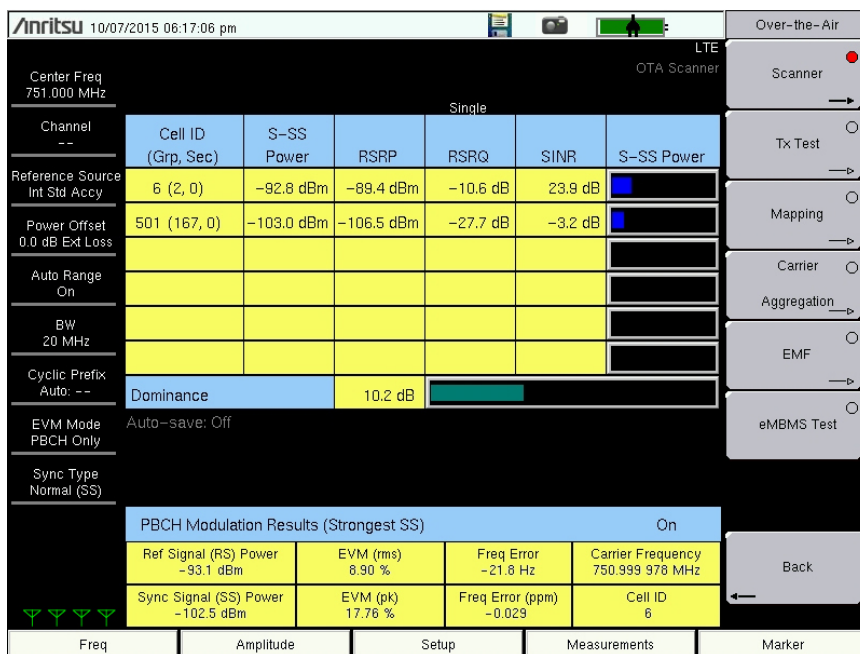
Figure 5-12. Over-the-Air Scanner Measurements
