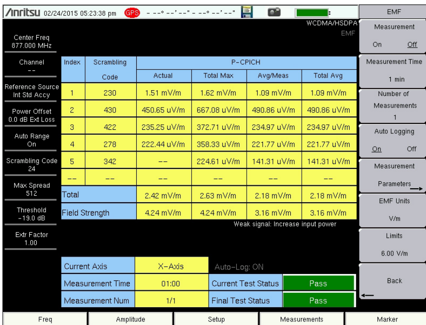
Figure 9-13. W-CDMA EMF Measurement Results
