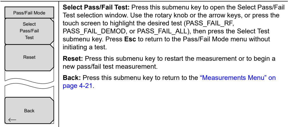
Figure 4-25. TD-SCDMA/HSDPA Pass Fail Mode Menu
