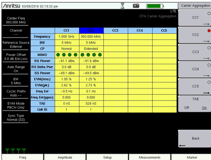
Figure 5-14. Over-the-Air Carrier Aggregation Measurement
