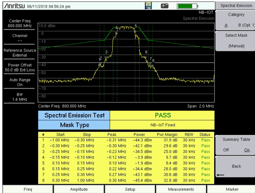
Figure 8-5. NB-IoT Spectral Emission Mask Display
