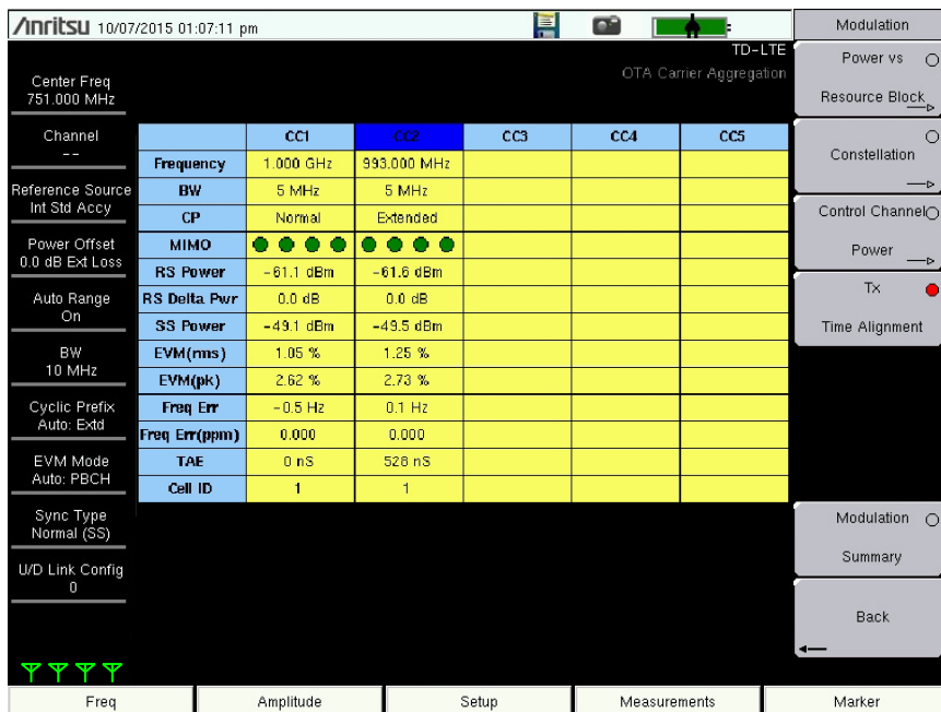
Figure 6-15. Over-the-Air Carrier Aggregation Measurement
