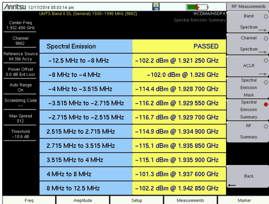
Figure 3-6. Spectral Emission Mask Summary
