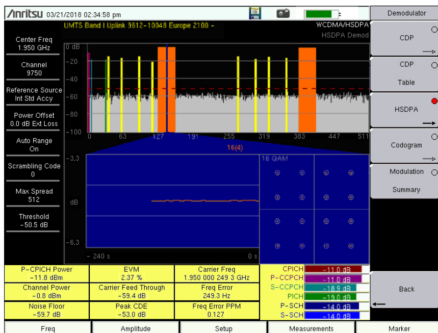
Figure 3-9. HSDPA Measurement Summary
