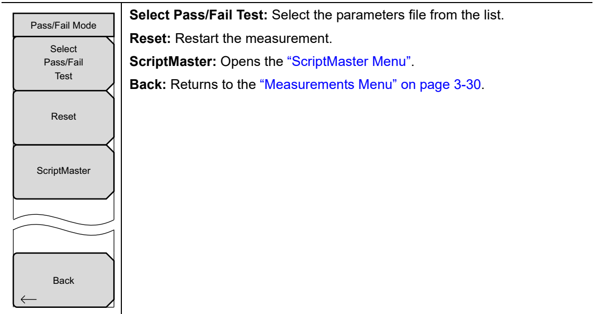
Figure 3-32. W-CDMA/HSDPA Pass/Fail Mode Menu
