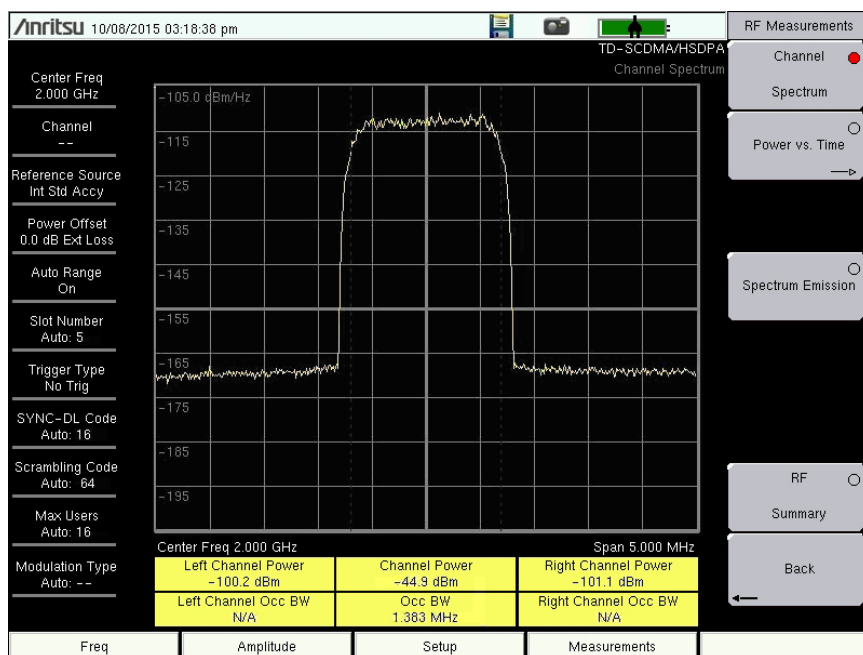
Figure 4-1. TD-SCDMA/HSDPA Channel Spectrum
