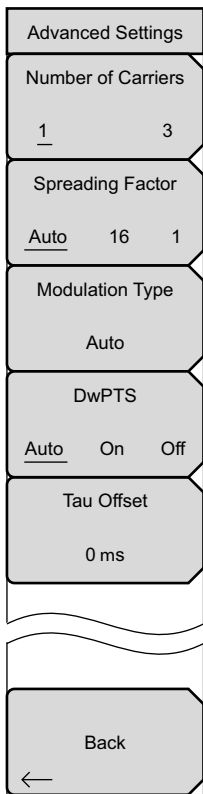
Figure 4-18. TD-SCDMA/HSDPA Advanced Settings Menu
