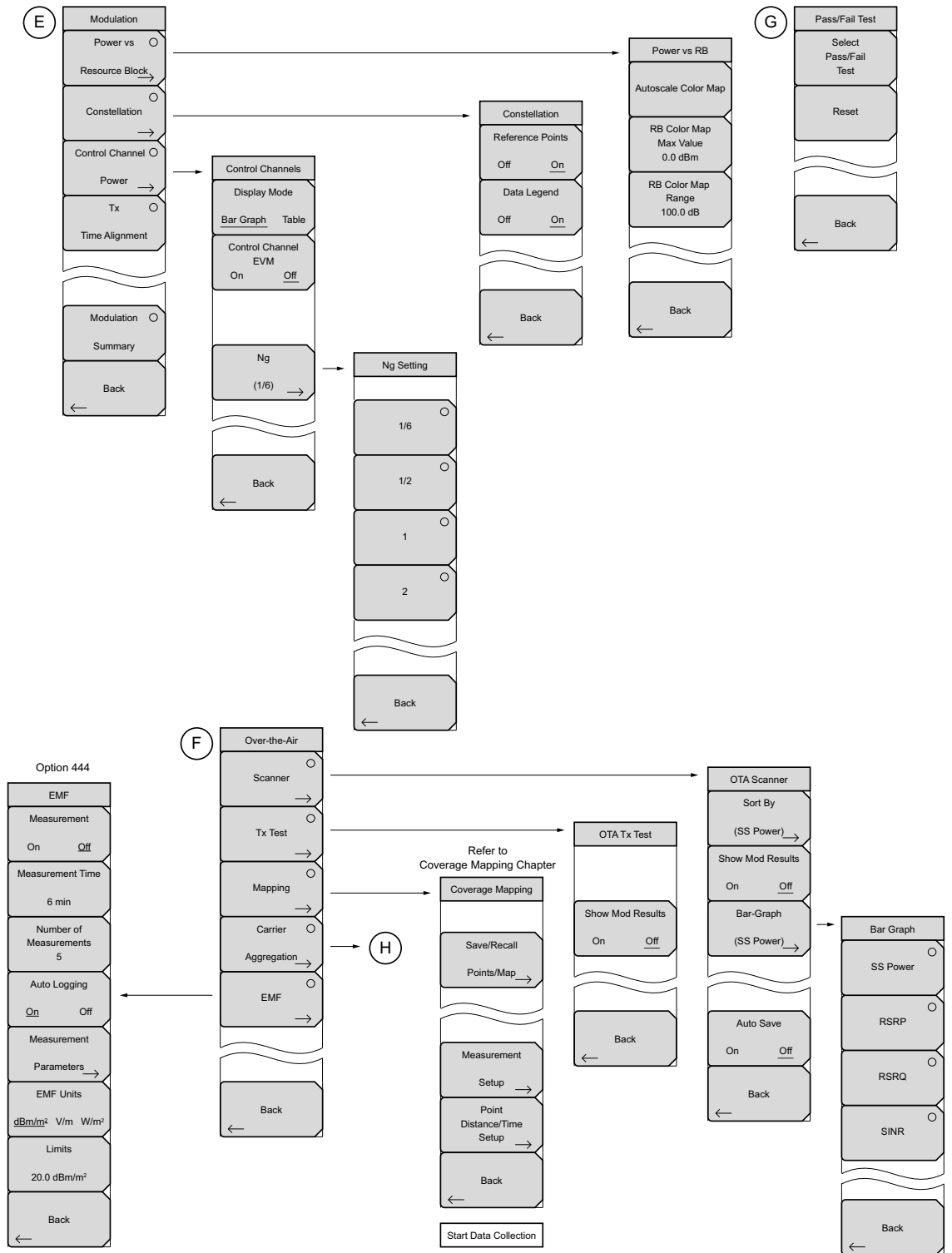
Figure 6-19. TD-LTE Menu Layout (2 of 3)
