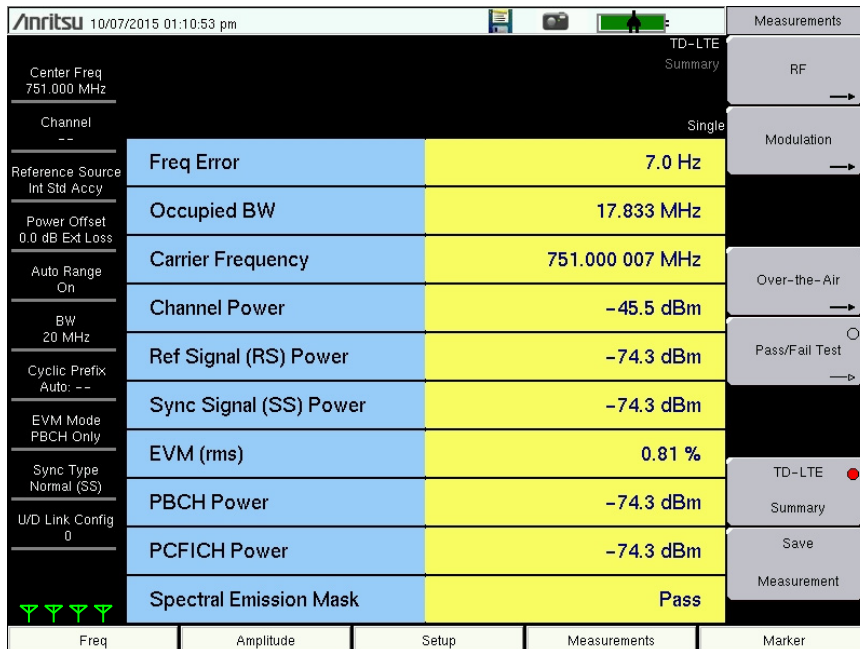
Figure 6-17. TD-LTE Summary
