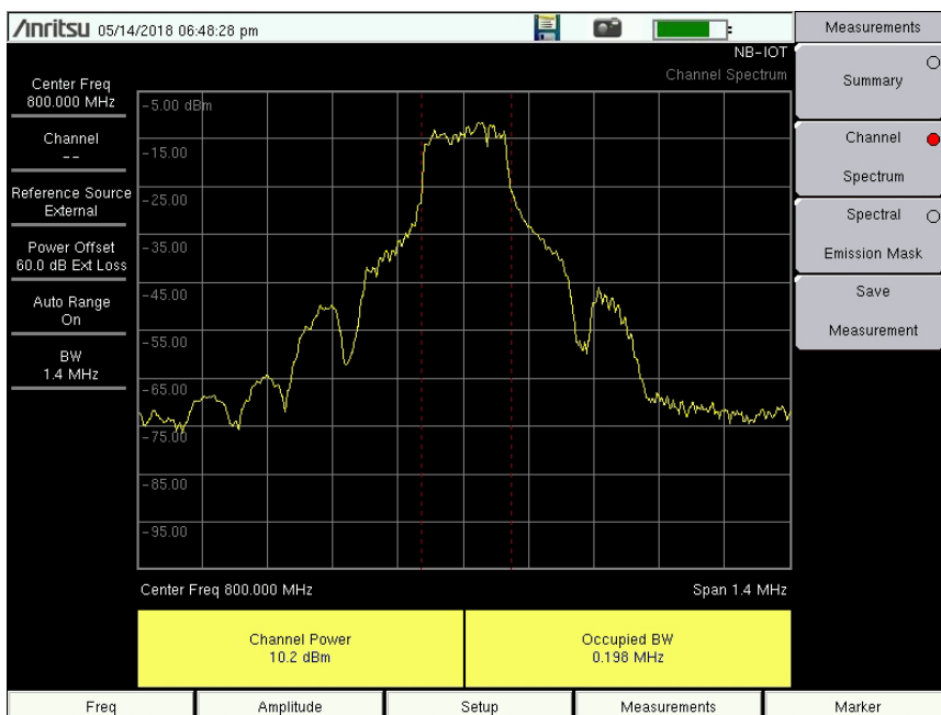
Figure 8-3. NB-IoT Channel Spectrum Display
