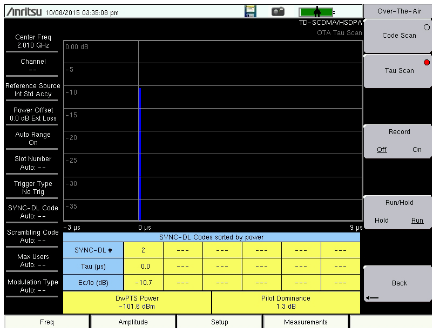
Figure 4-6. TD-SCDMA/HSDPA OTA Tau Scan
