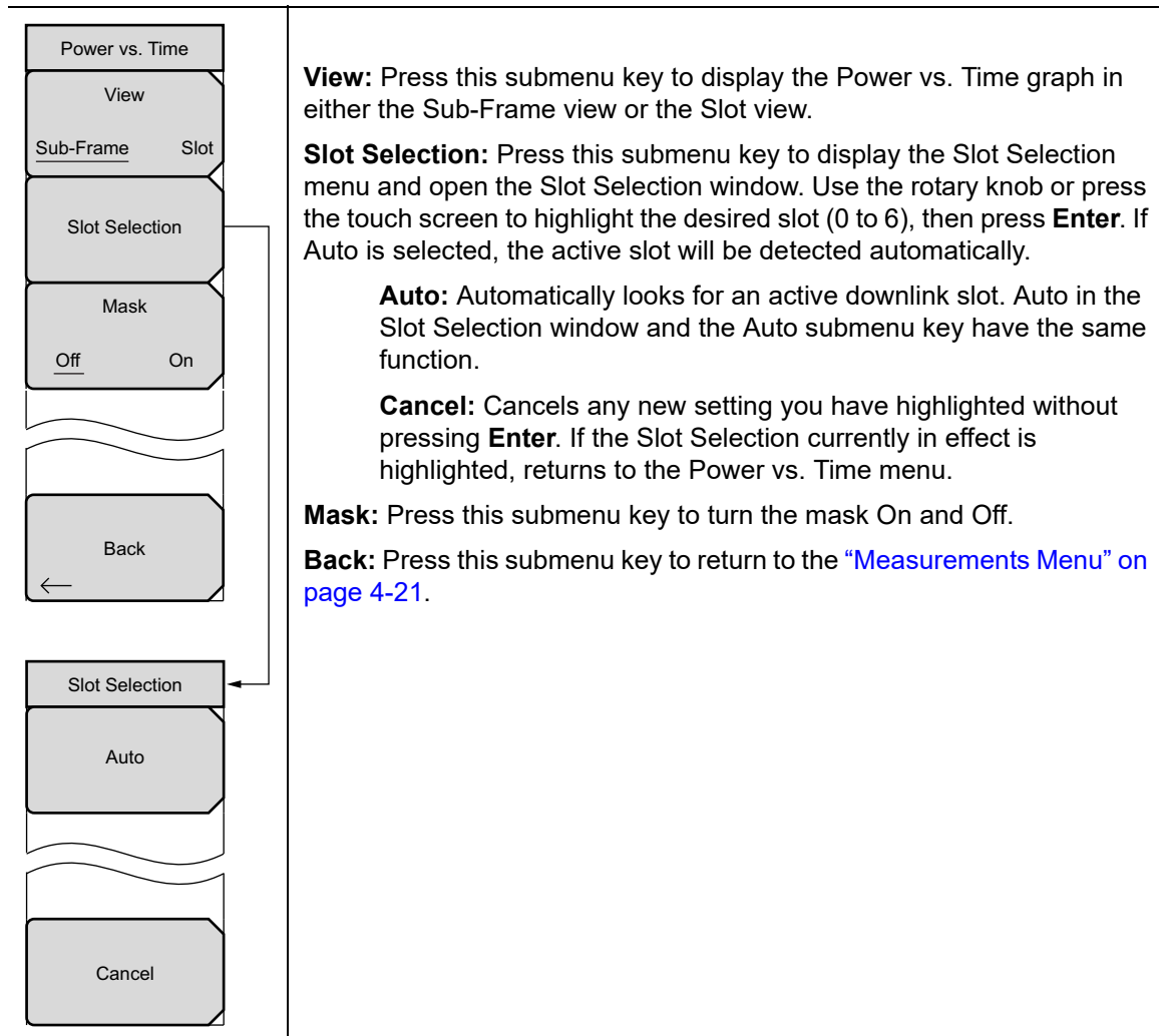
Figure 4-22. TD-SCDMA/HSDPA Power vs. Time Menu
