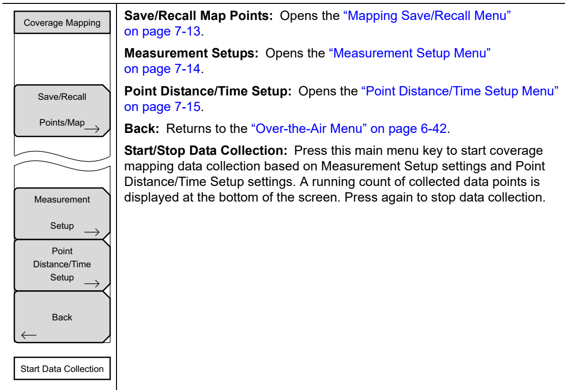
Figure 6-40. Coverage Mapping Menu
