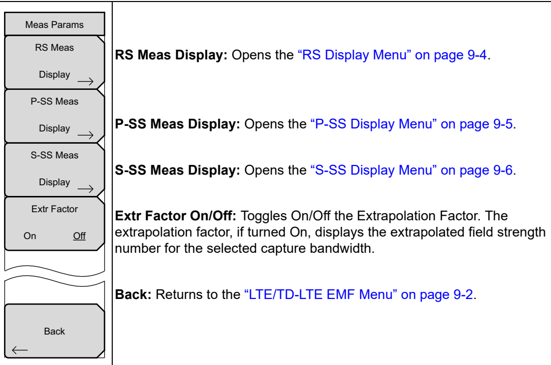
Figure 9-3. LTE/TD-LTE Meas Params Menu
