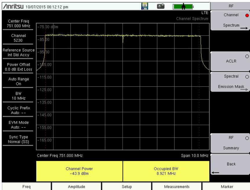
Figure 5-2. Channel Spectrum
