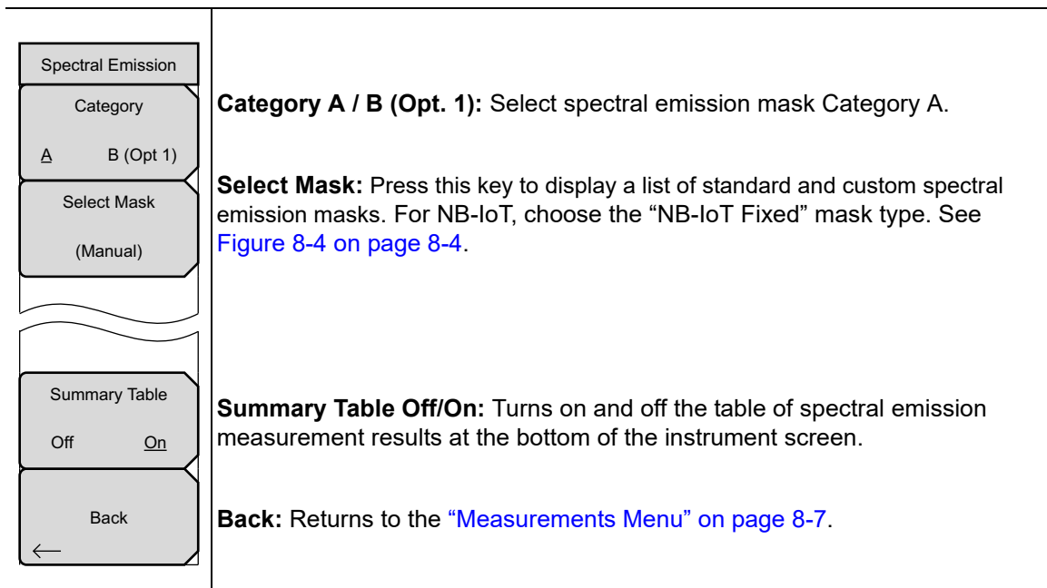
Figure 8-10. Spectral Emission Menu
