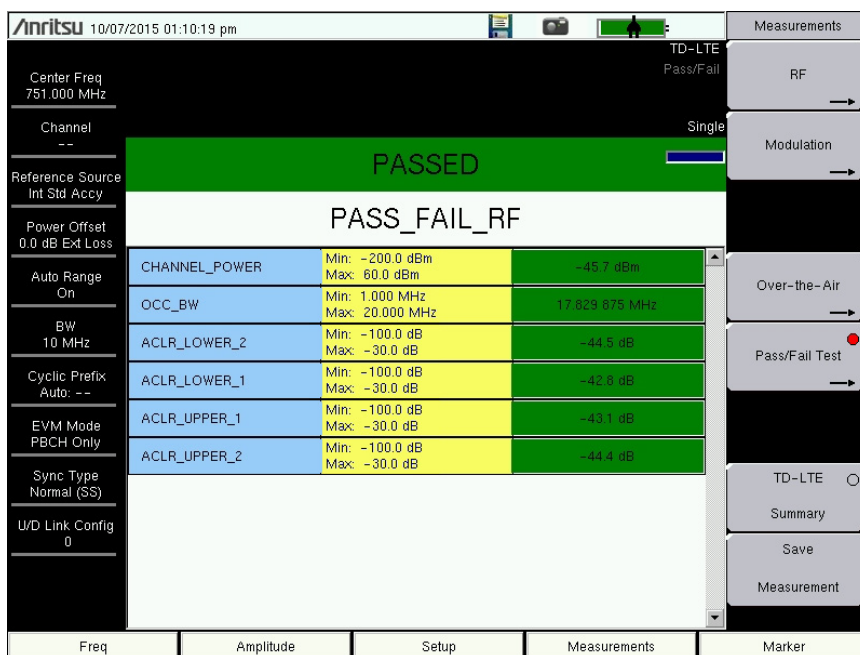
Figure 6-16. Past/Fail Test
