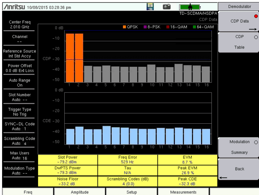
Figure 4-4. TD-SCDMA/HSDPA Demodulator, CDP Data
