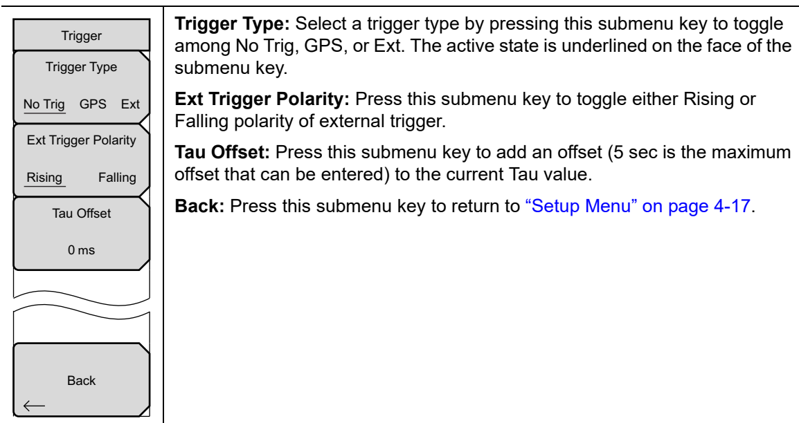
Figure 4-14. TD-SCDMA/HSDPA Trigger Menu
