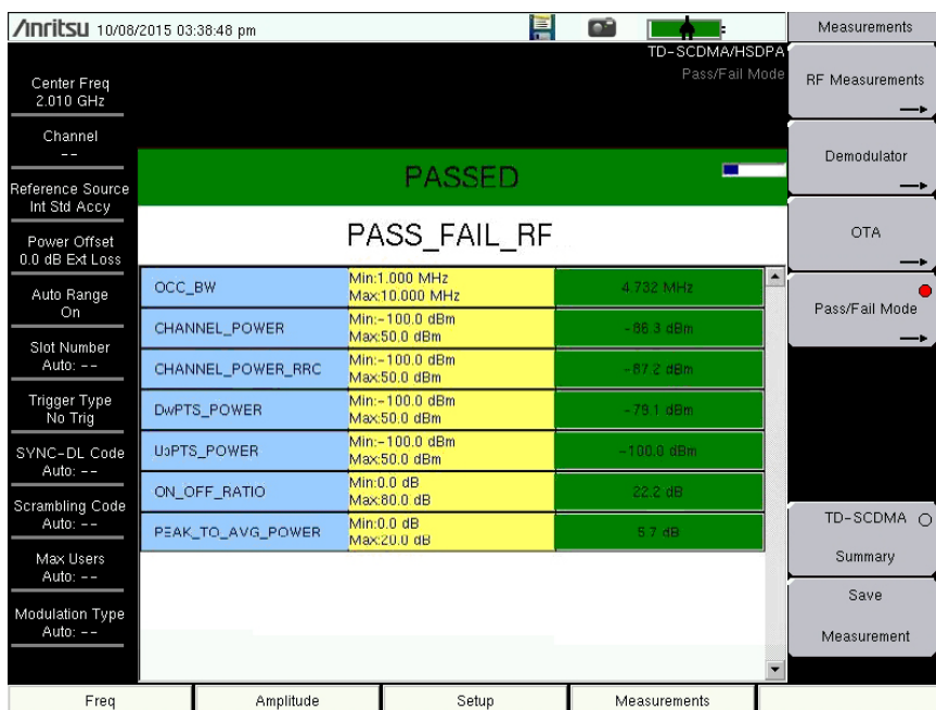
Figure 4-7. TD-SCDMA/HSDPA Pass/Fail Measurements
