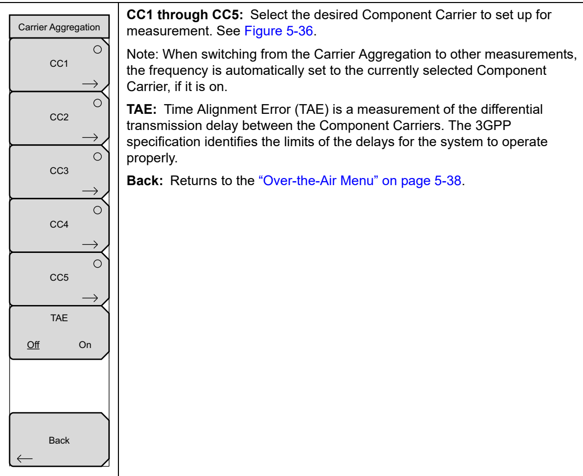
Figure 5-35. Carrier Aggregation Menu
