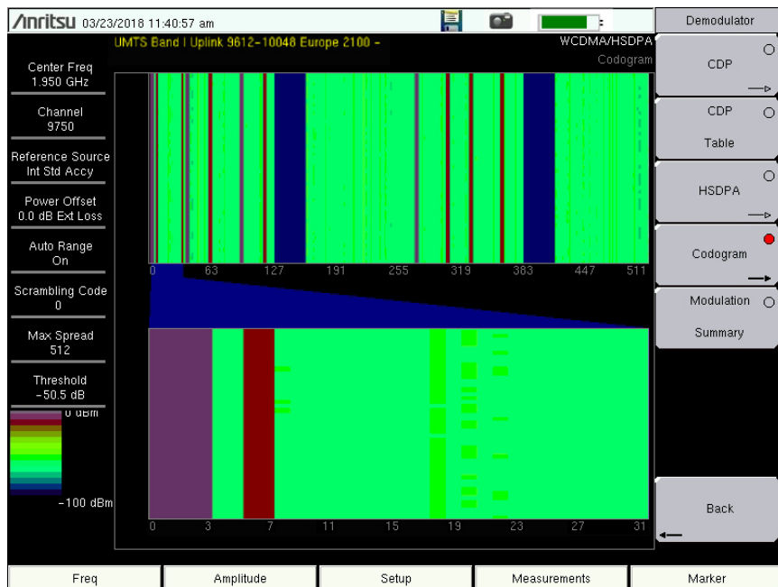
Figure 3-10. Codogram Measurement
