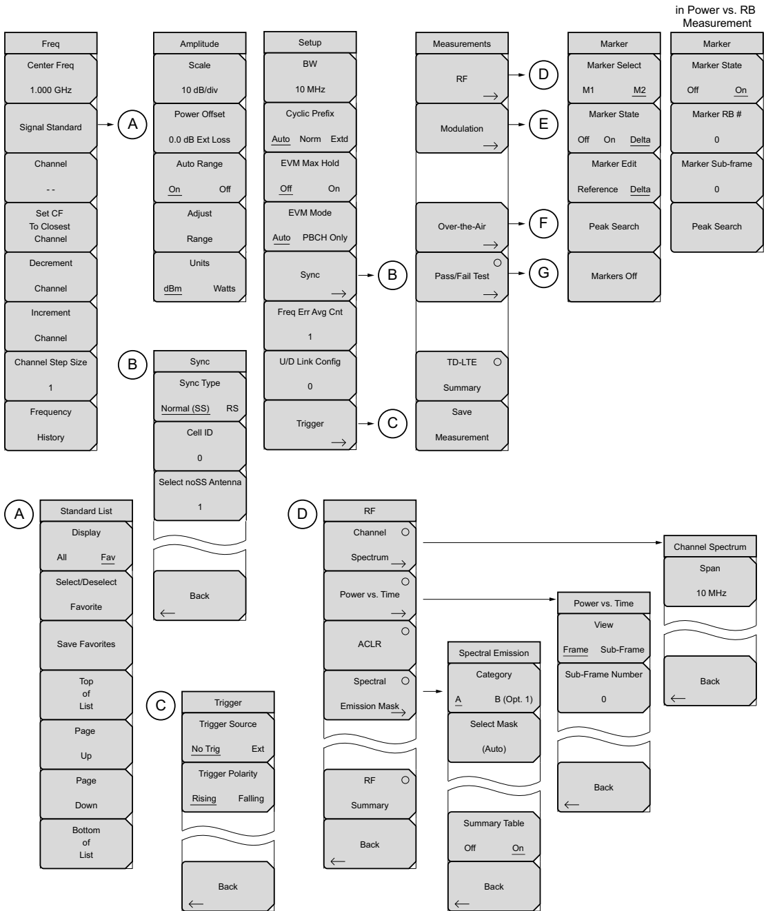
Figure 6-18. TD-LTE Menu Layout (1 of 3)
