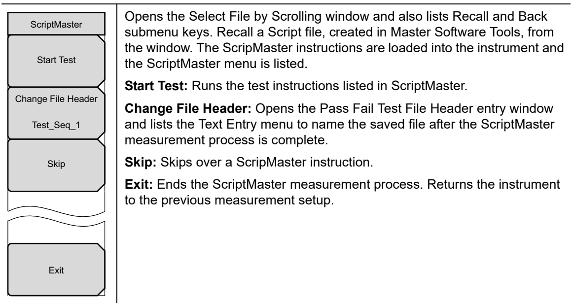
Figure 3-33. W-CDMA/HSDPA ScriptMaster Menu
