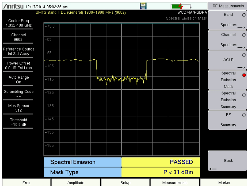
Figure 3-5. Spectral Emission Mask Measurement
