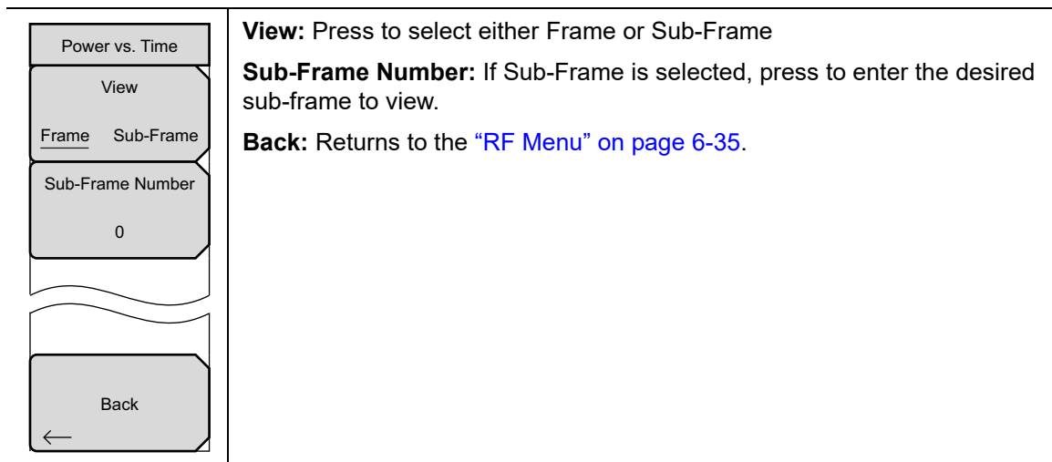
Figure 6-31. TD-LTE Power vs. Time Menu
