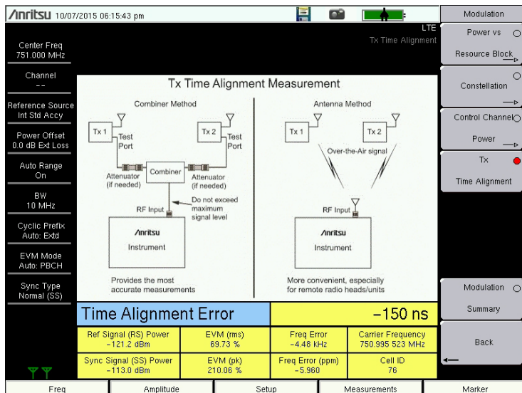
Figure 6-11. Tx Time Alignment
