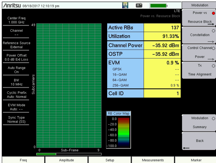
Figure 5-6. Power versus Resource Block Measurement View
