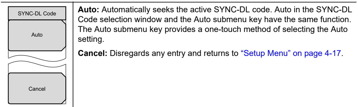
Figure 4-15. TD-SCDMA/HSDPA Trigger Menu
