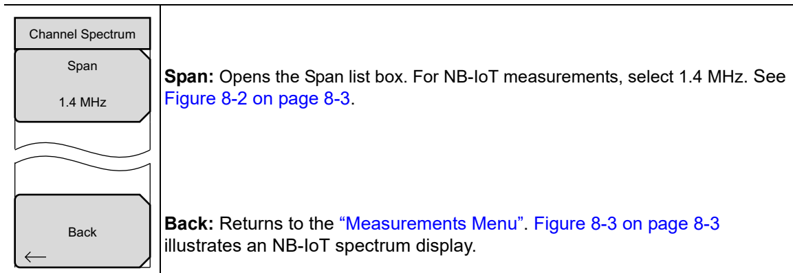
Figure 8-9. Channel Spectrum Menu
